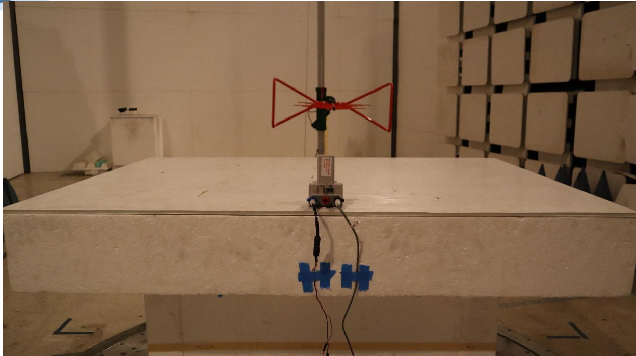
Digital Emissions ERW-1350-001, 30MHz-1GHz, Front
