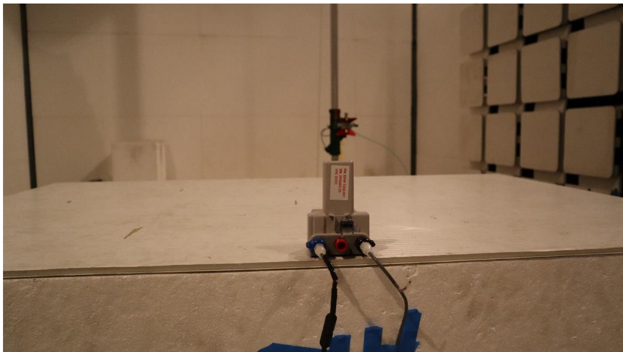
Digital Emissions ERW-1350-001, 1-18GHz, Front
