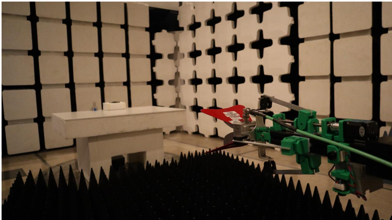
Digital Emissions ERW-1350-001, External Antenna, 1-18GHz, Back
