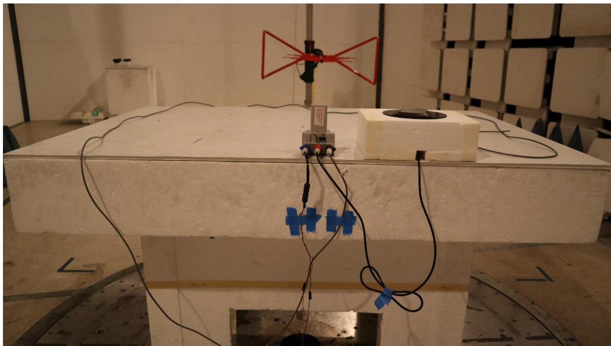
ERW-1350-001 External Antenna, 30MHz-1GHz, Front
