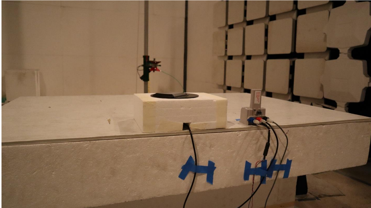
Digital Emissions ERW-1350-001 External Antenna, 1-18GHz, Front
