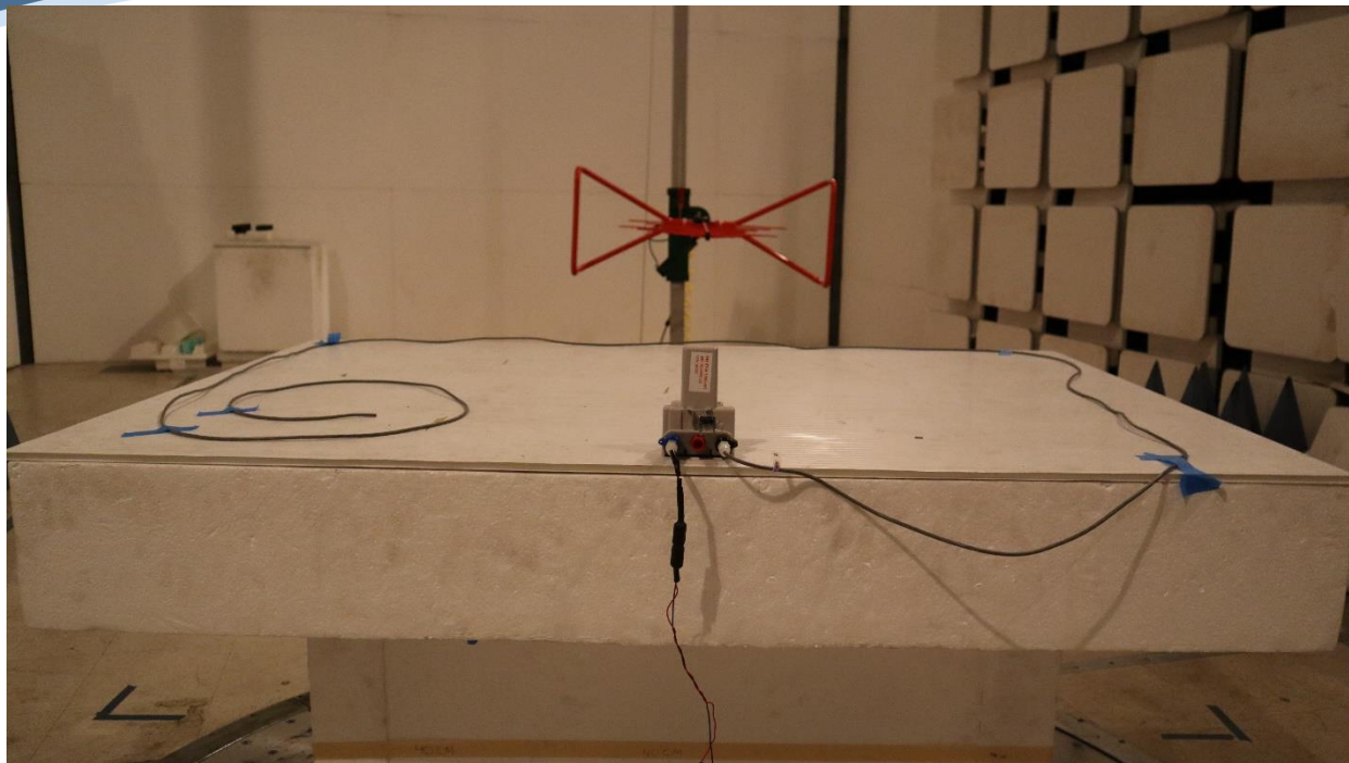
ERW-1350-001, 30MHz-1GHz, Front
