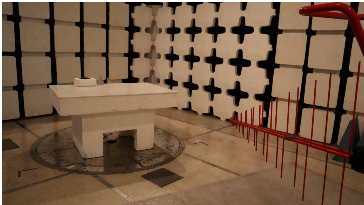
Digital Emissions ERW-1350-001 External Antenna, 30MHz-1GHz, Back
