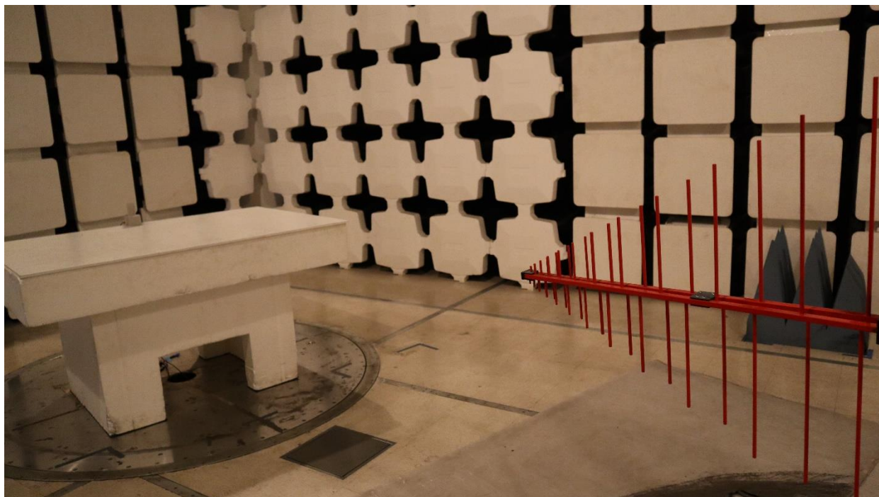
Digital Emissions ERW-1350-001, 30MHz-1GHz, Back
