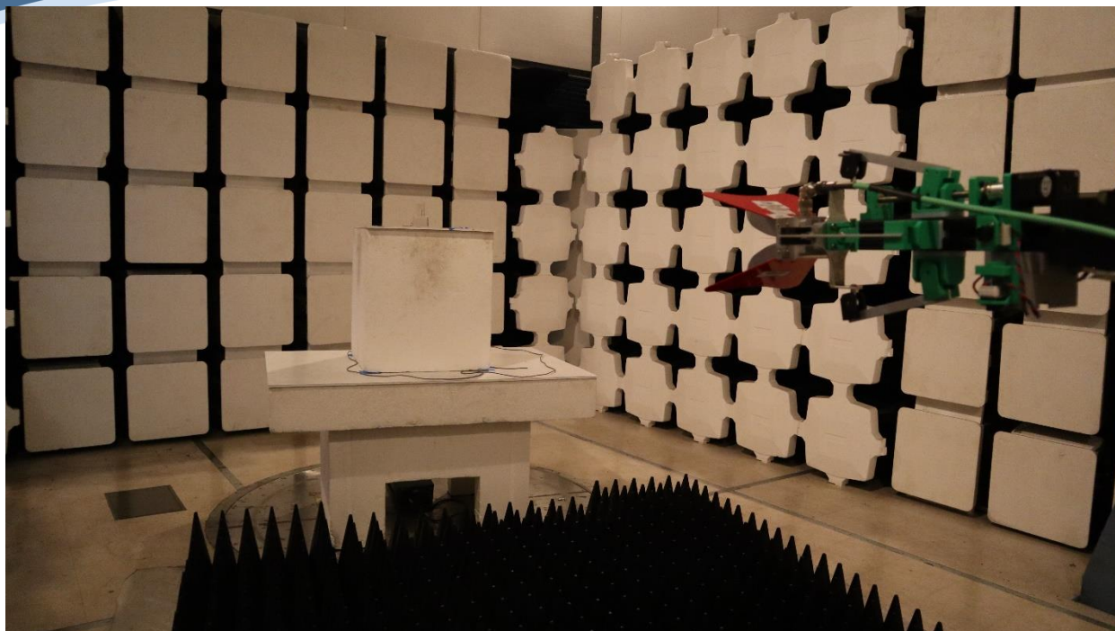
Spurious Emissions ERW-1350-001, 1-18GHz, Back
