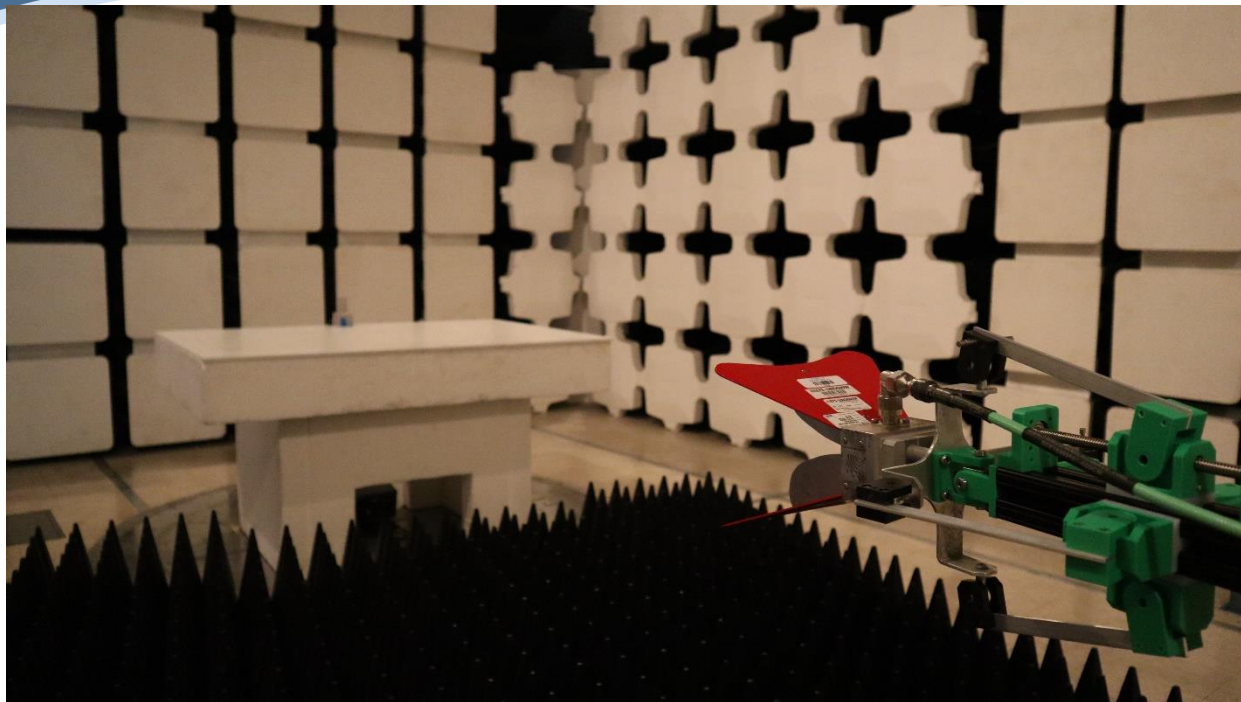
Digital Emissions ERW-1350-001, 1-18GHz, Back
