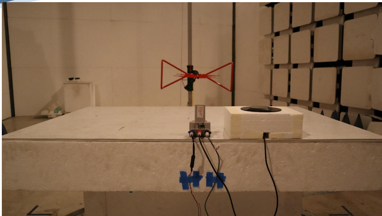
Digital Emissions ERW-1350-001 External Antenna, 30MHz-1GHz, Front
