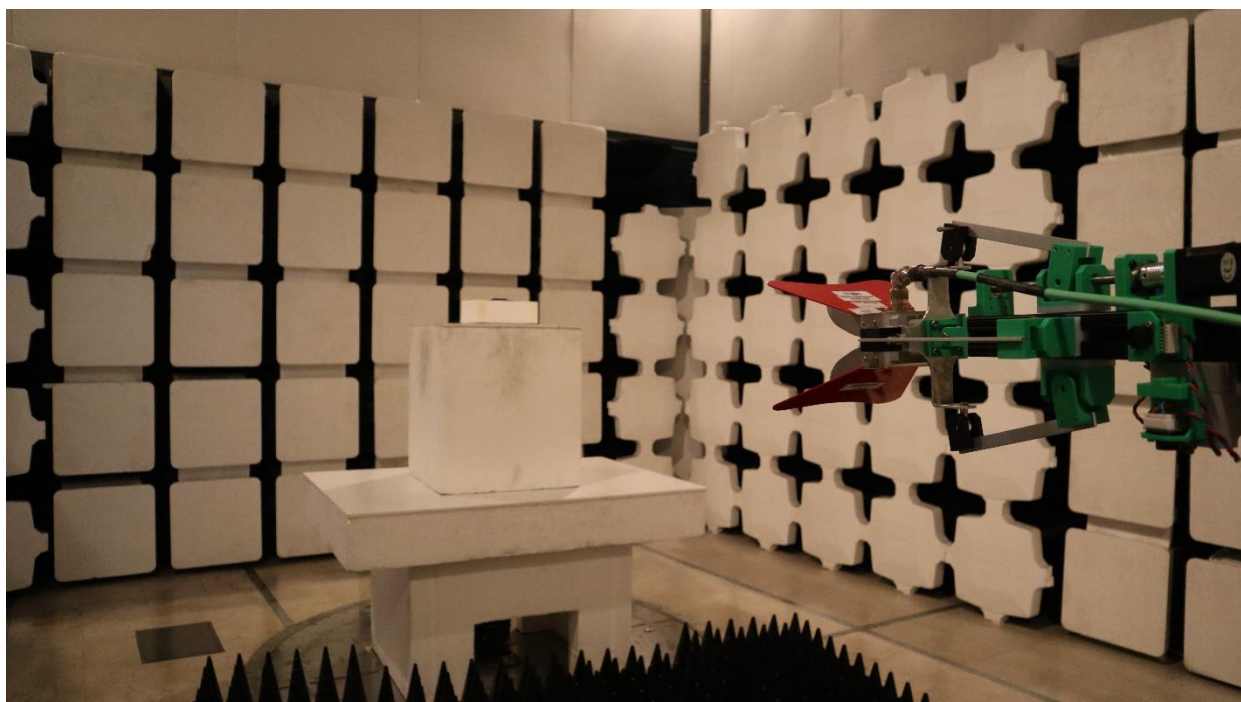
Spurious Emissions ERW-1350-001, External Antenna, 1-18GHz, Back
