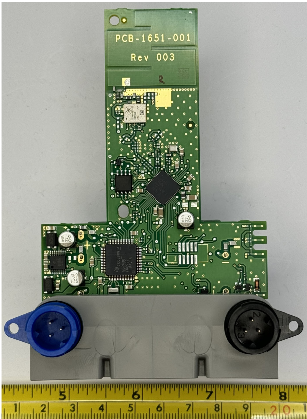
Figure 2.8: Pit 2-Port - Front
