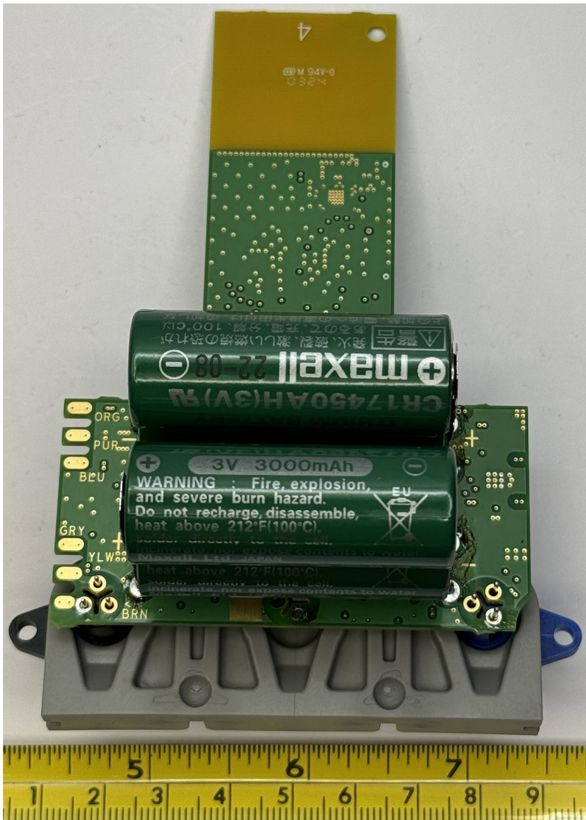
Figure 2.6: Pit 4-Battery, 2-Port - Back
