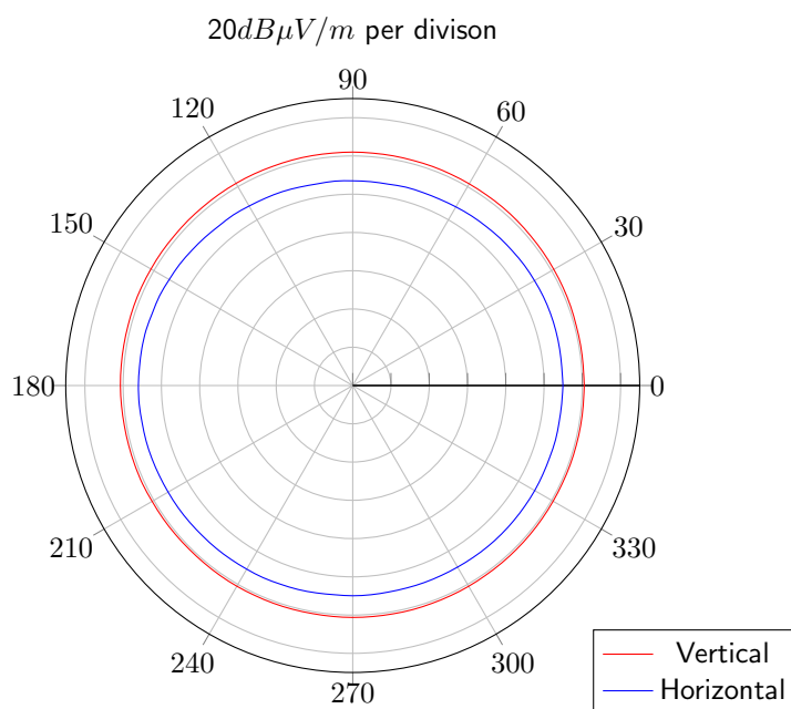
Figure 2: Radiation Pattern
