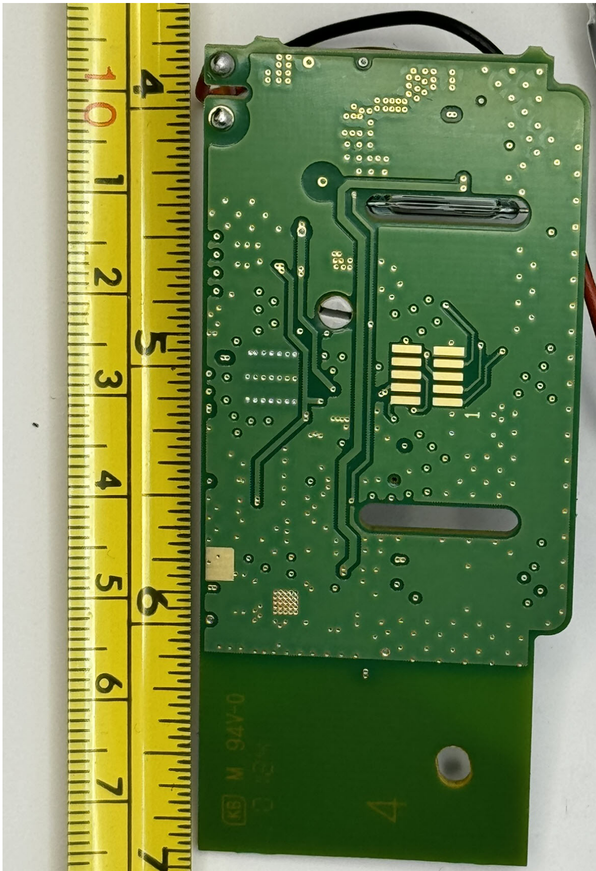
Figure 2.2: PCB Back
