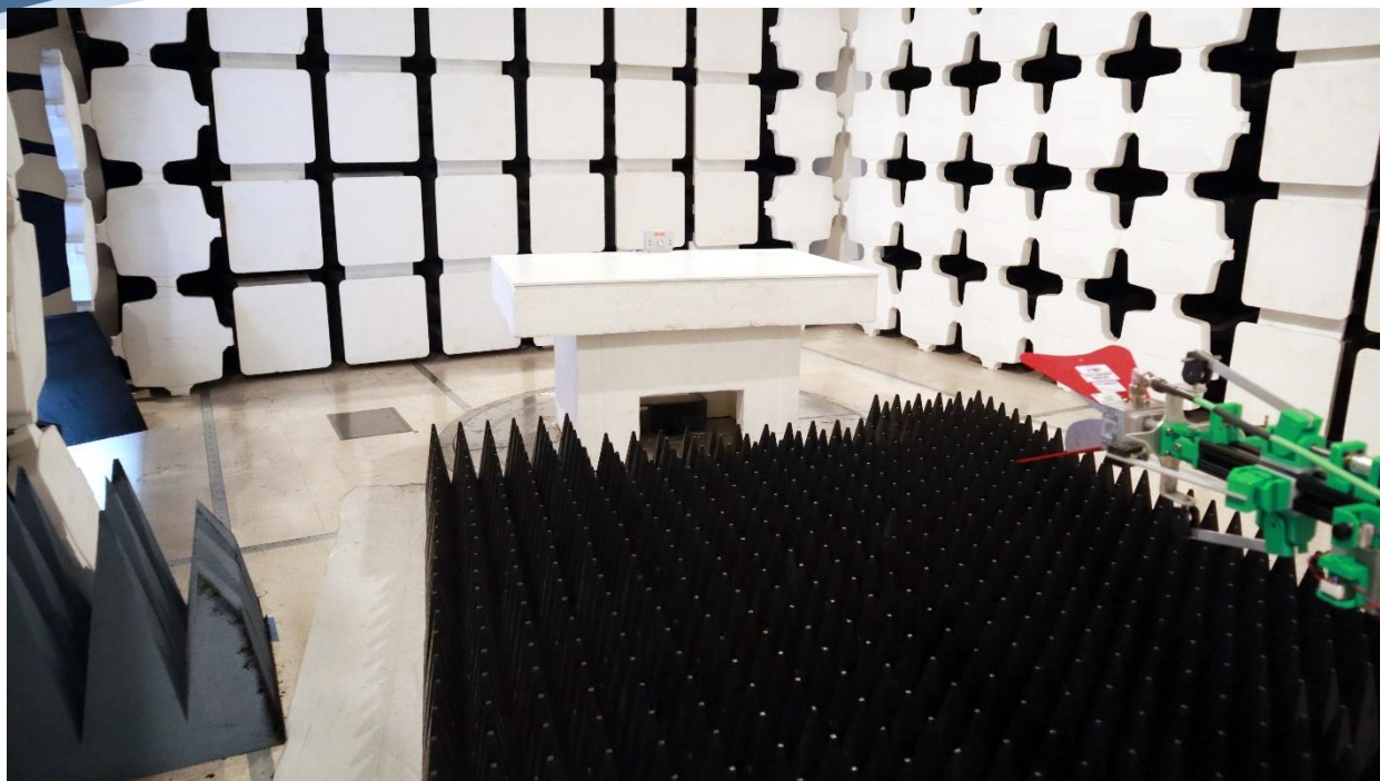
Digital Emissions ERG-5600-008, 1-18GHz Back, Power Cable Down
