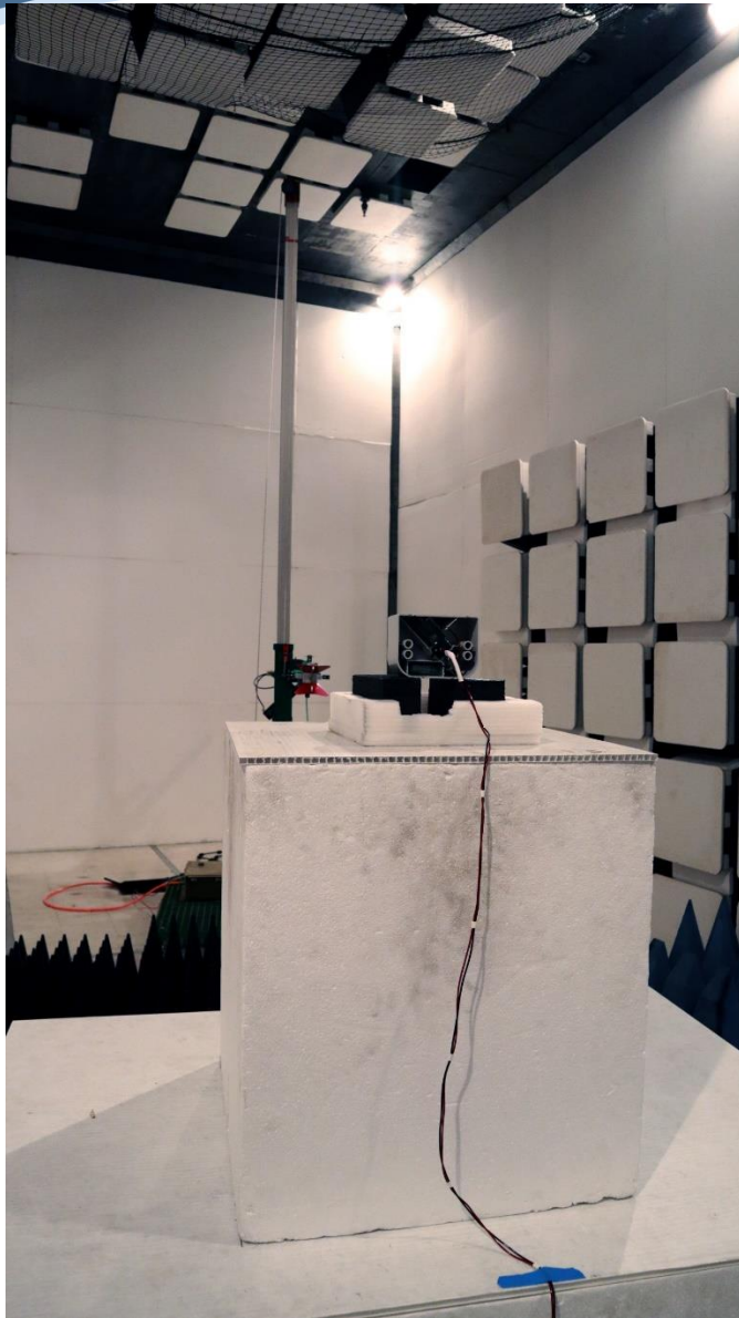
Spurious Emissions ERG-5600-008, 1-18GHz Front, Power Cable Down
