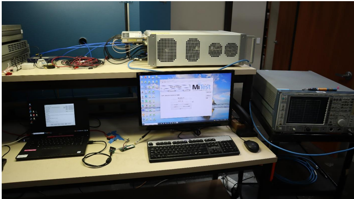
100G_Setup
