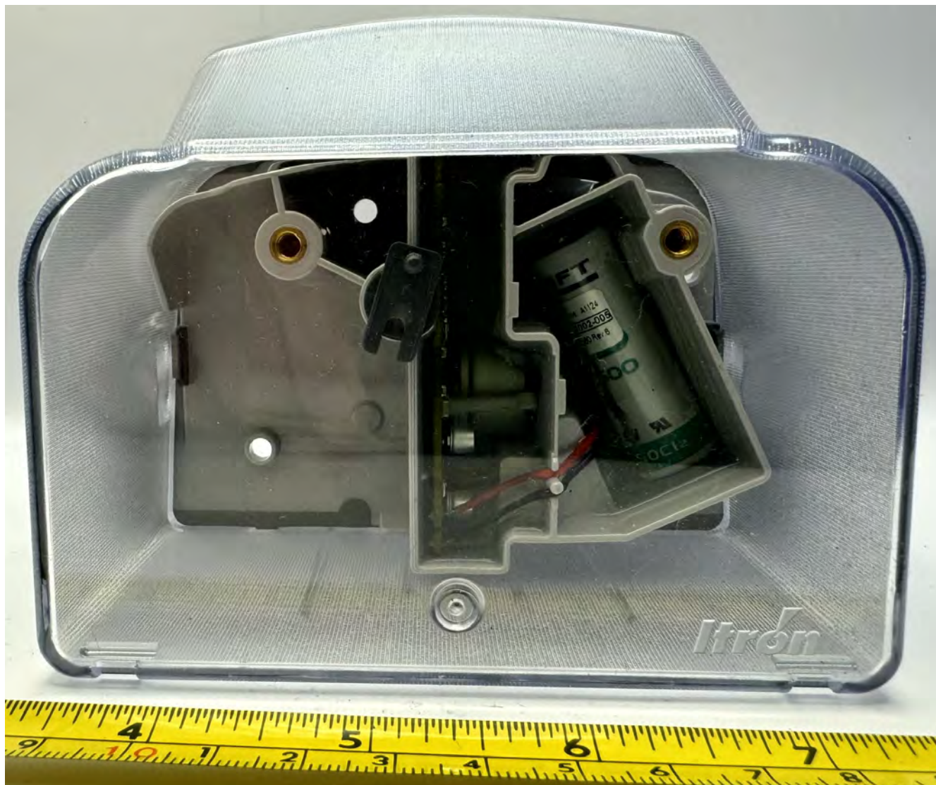
Figure 2.1: ERG-5600-005 External Front
