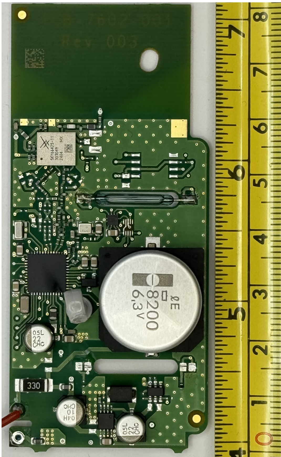
Figure 2.1: PCB Front
