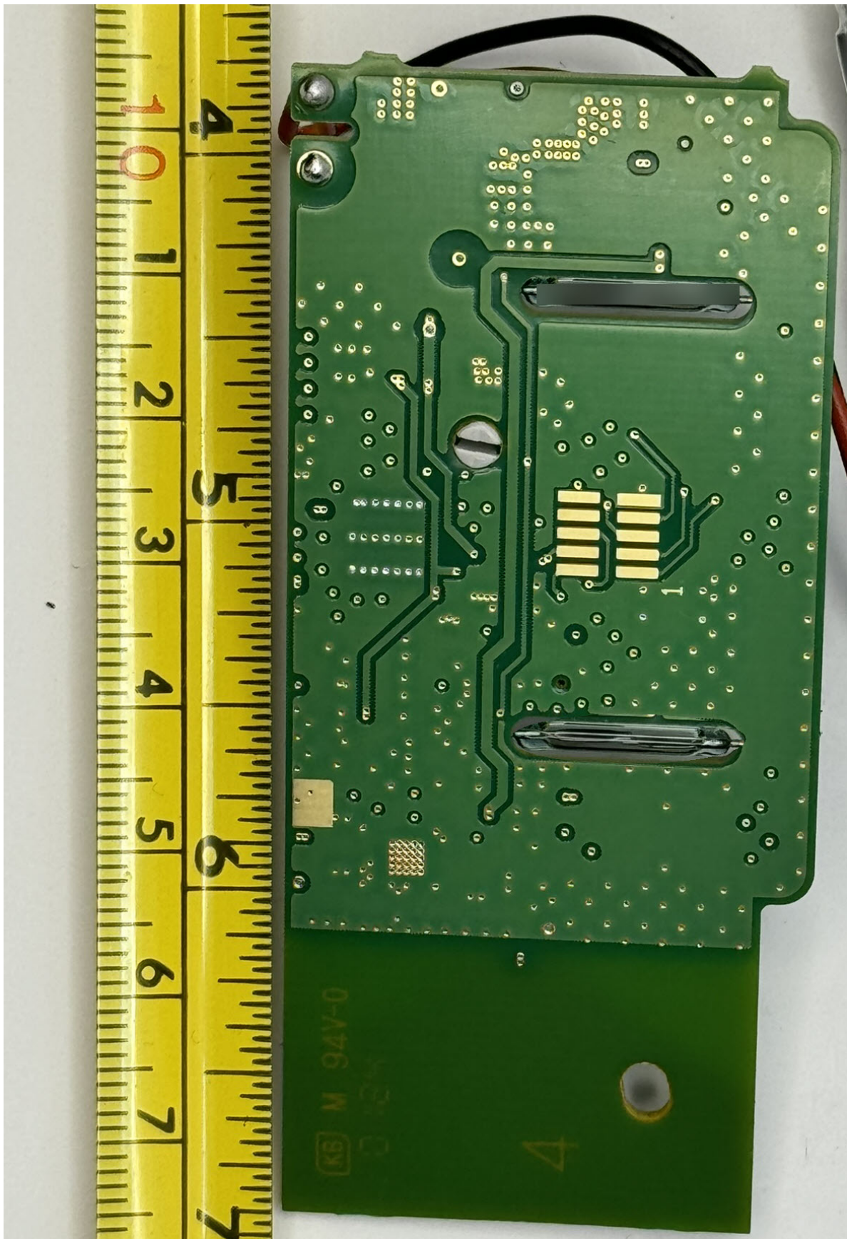
Figure 2.2: PCB Back
