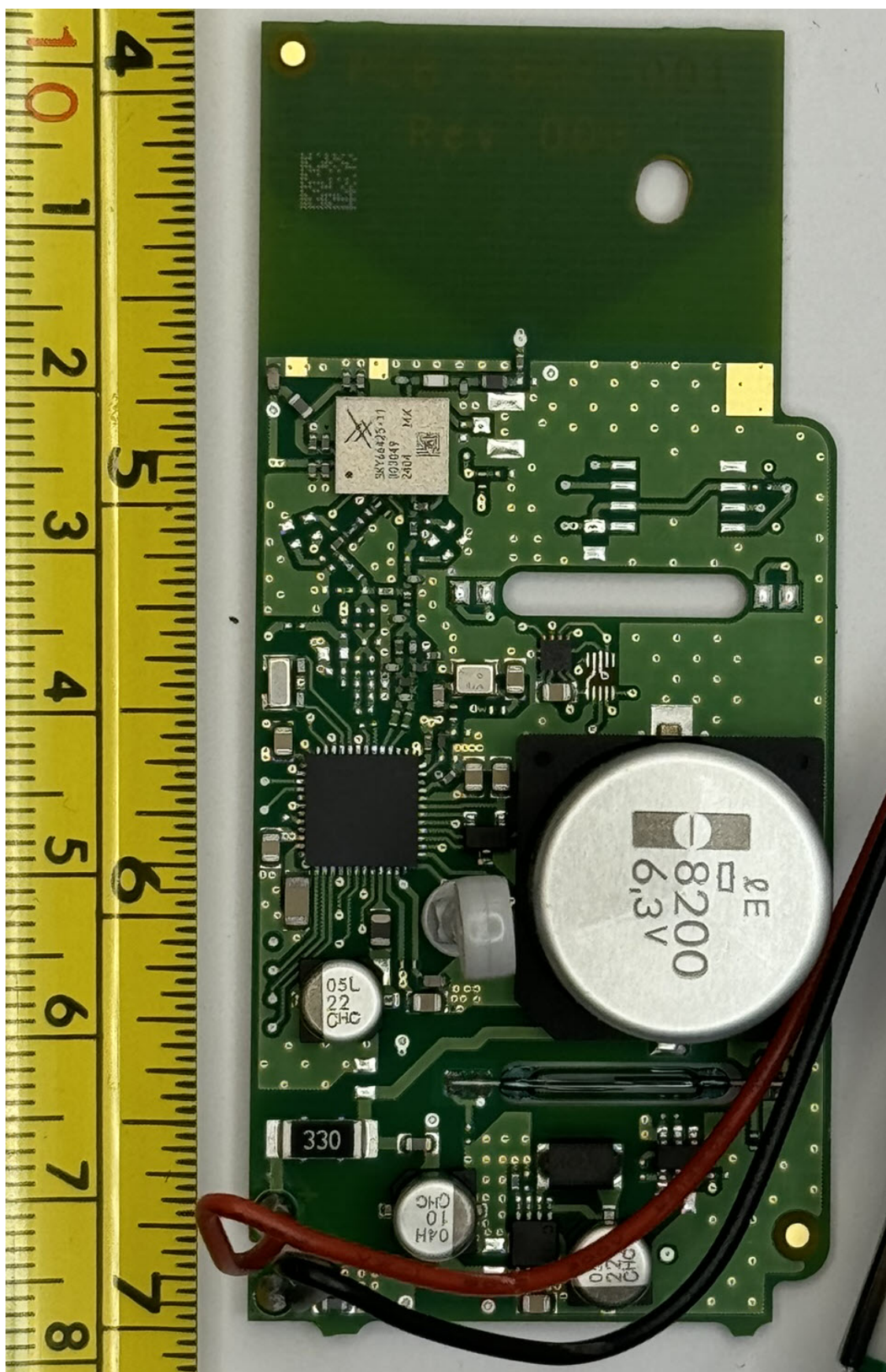
Figure 2.1: PCB Front
