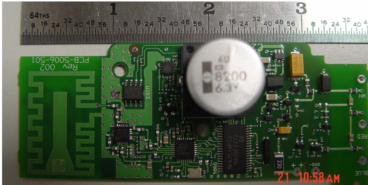
Top Side of PCB-5006-501 used in 100GDLRS
