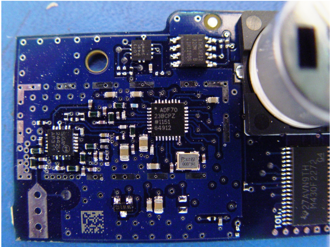
Printed circuit board assembly used in ERG-5006-501 Top Side (RF section).
