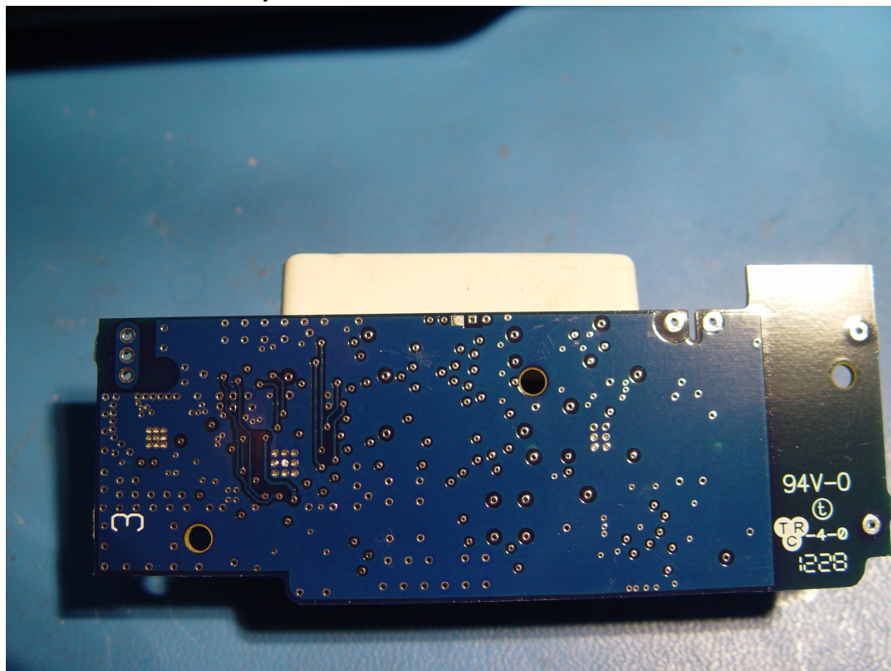
Printed circuit board assembly used in ERG-5006-501 Bottom Side.
