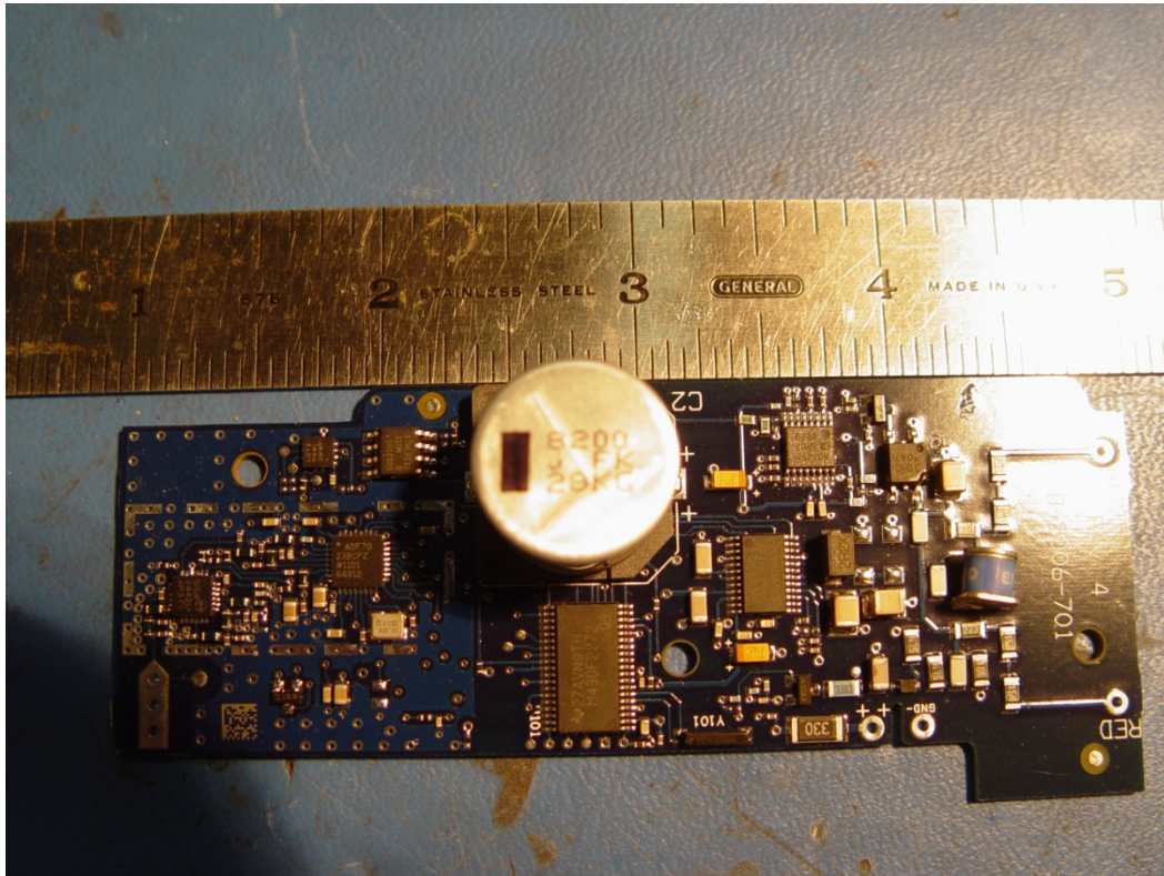
Printed circuit board assembly used in ERG-5006-501 height view.
