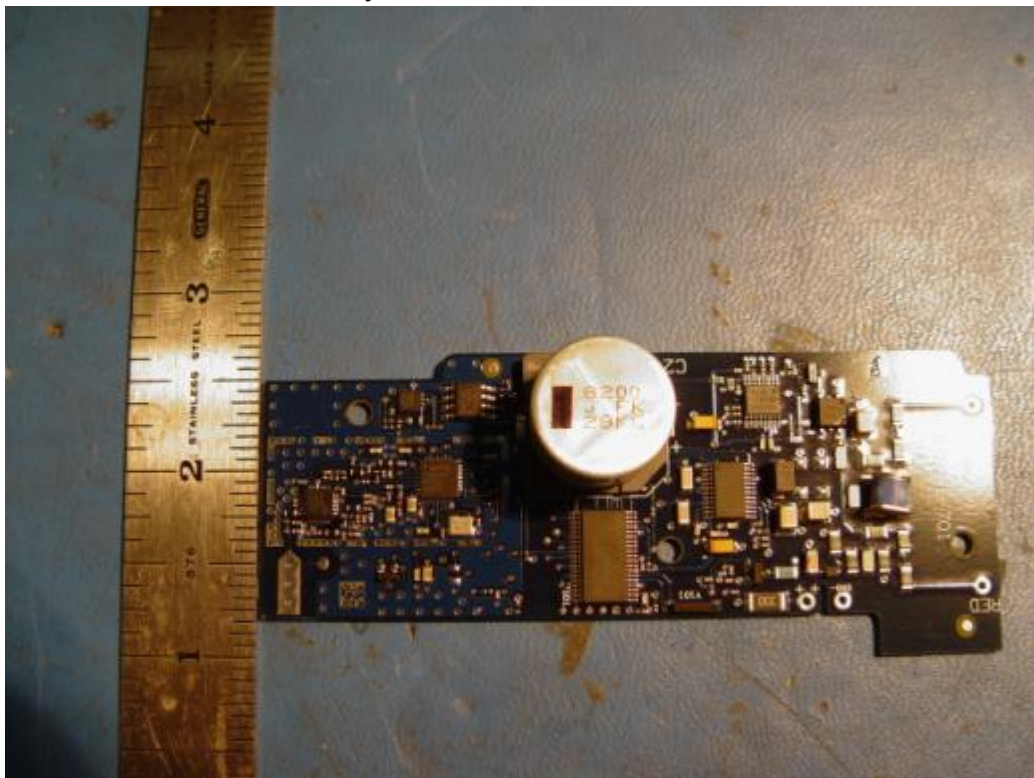
Printed circuit board assembly used in ERG-5006-501 width view.
