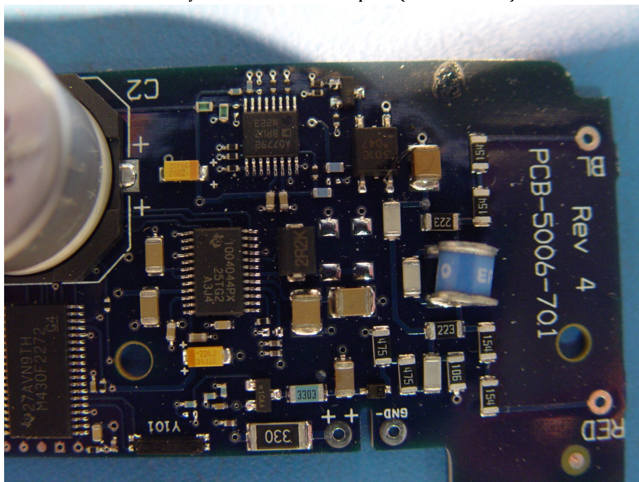
Printed circuit board assembly used in ERG-5006-501 Top Side (interface section).
