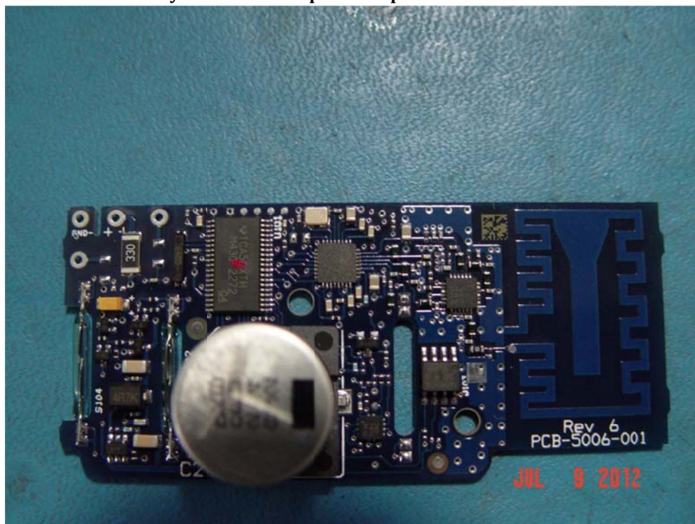
Printed circuit board assembly used in all Endpoints Top side view.
