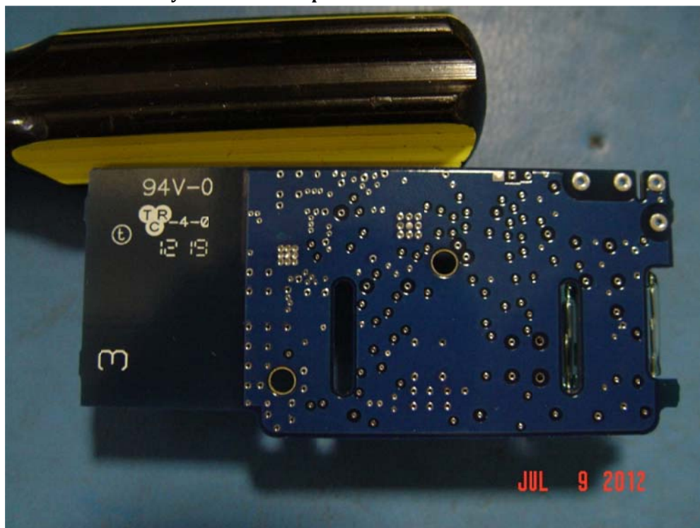
Printed circuit board assembly used in all Endpoints Bottom side view.
