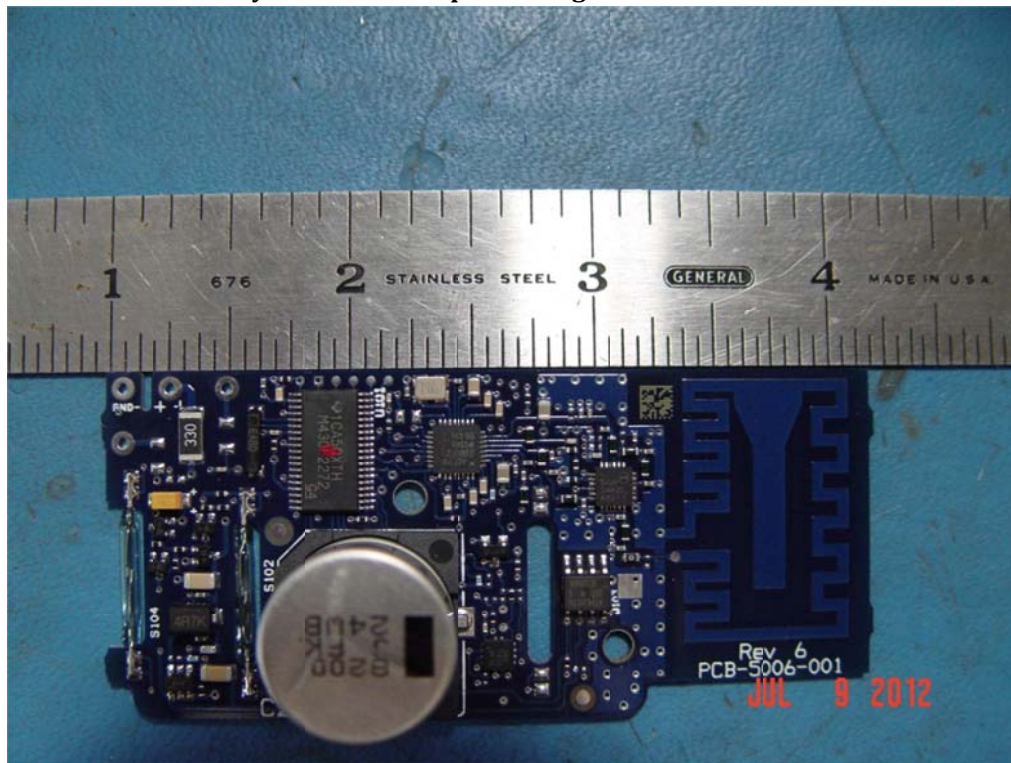
Printed circuit board assembly used in all Endpoints height view.
