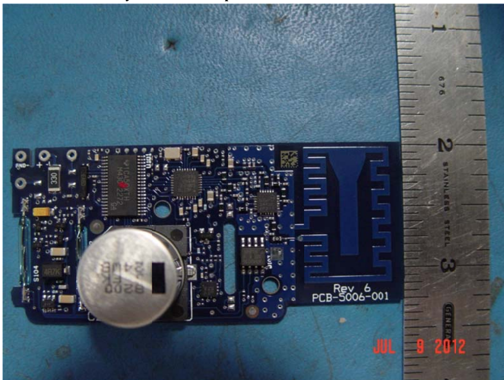
Printed circuit board assembly used in all Endpoints width view.
