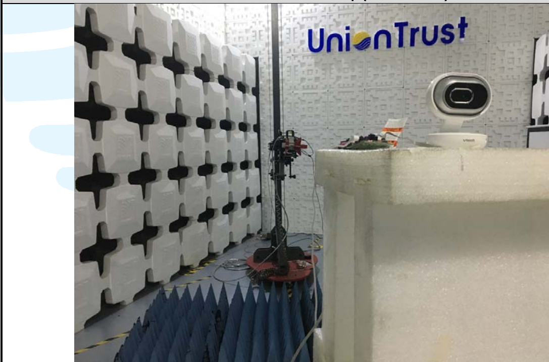
Radiated emission Test Setup (Above 1 GHz)
