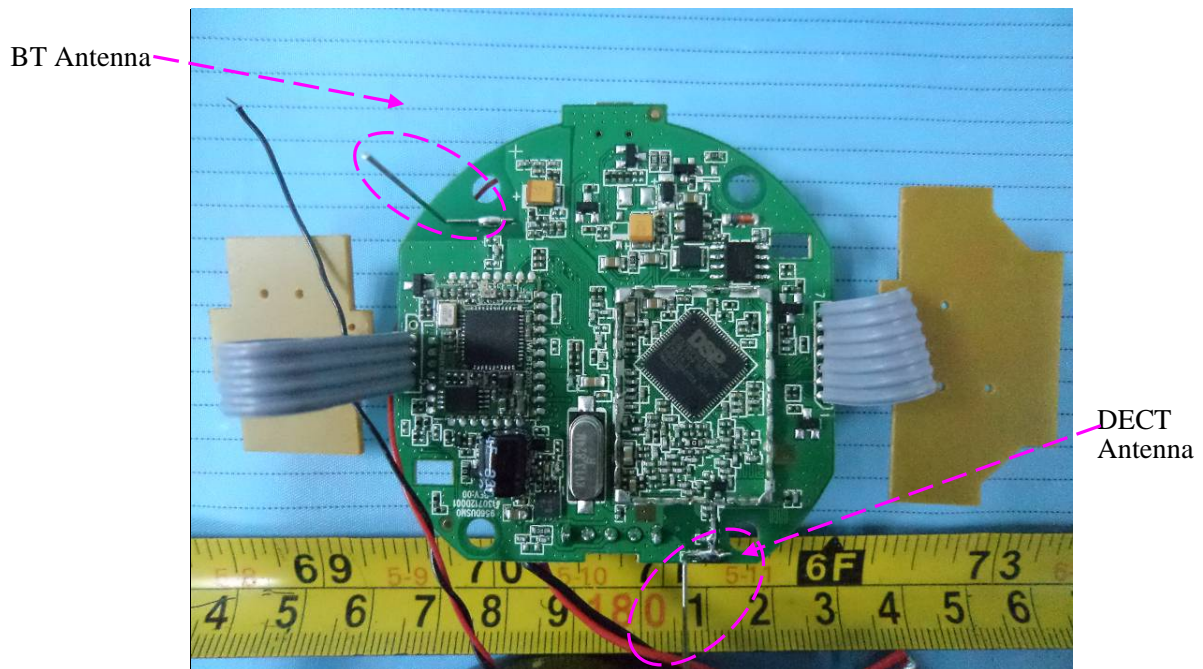
EUT – Main Board Top Shielding off View
