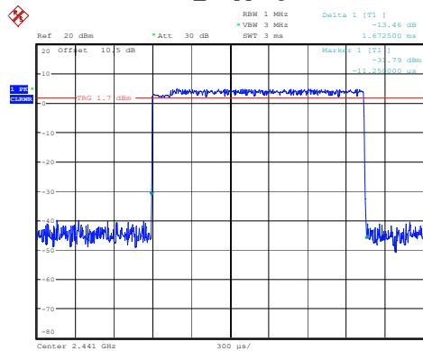
2DH3_Hopping 1.673ms
