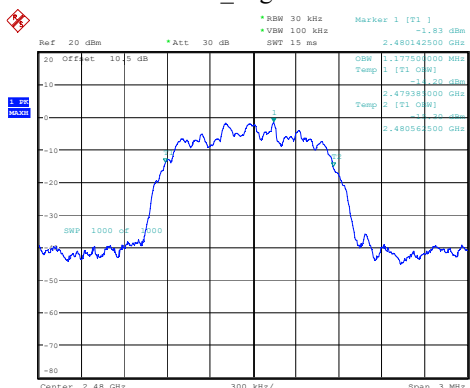
2DH1_High 1.178MHz
