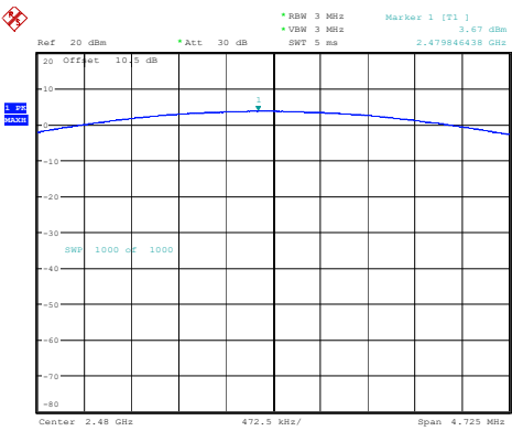
DH1_High 3.67dBm
