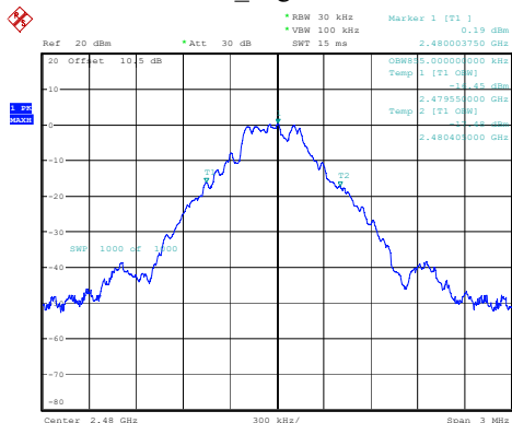
DH1_High 0.855MHz
