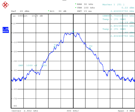
DH1_Low 0.859MHz
