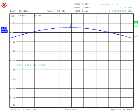
2DH1_Low 5.02dBm
