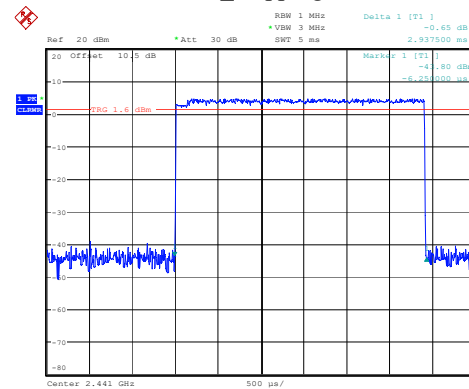
2DH5_Hopping 2.938ms
