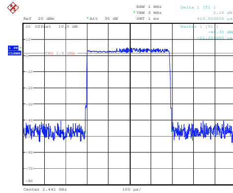
2DH1_Hopping 0.410ms
