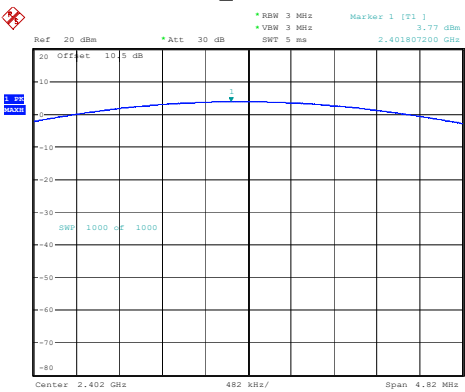
DH1_Low 3.77dBm
