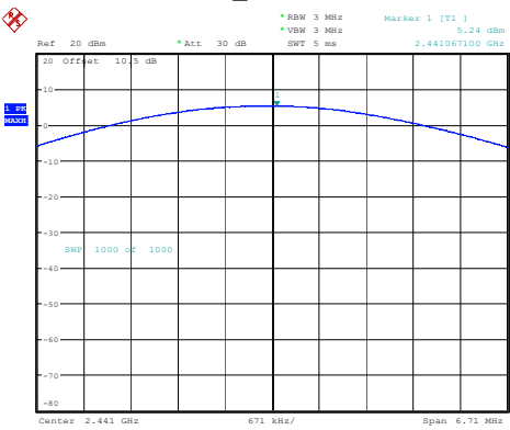
2DH1_Middle 5.24dBm
