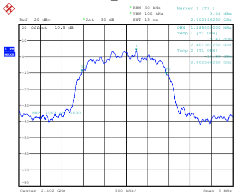
2DH1_Low 1.185MHz
