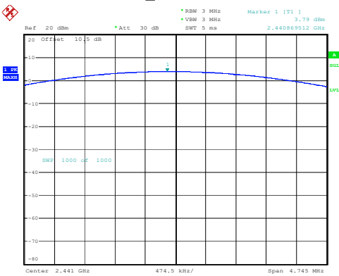
DH1_Middle 3.79dBm
