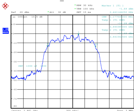
2DH1_Middle 1.178MHz
