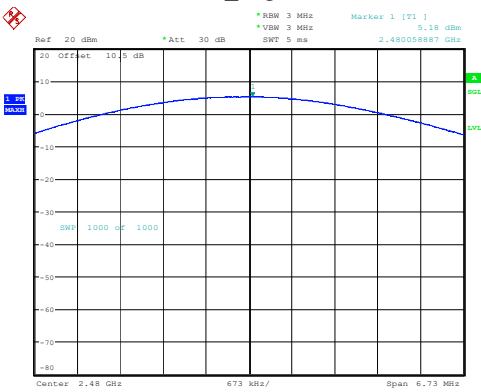
2DH1_High 5.18dBm
