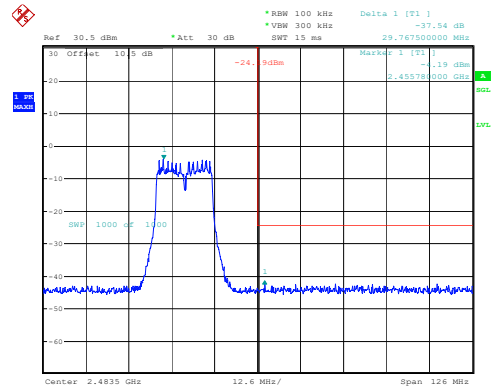
802.11g_2462MHz
