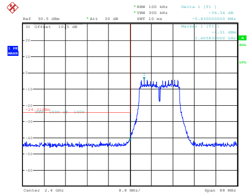
802.11g_2412MHz
