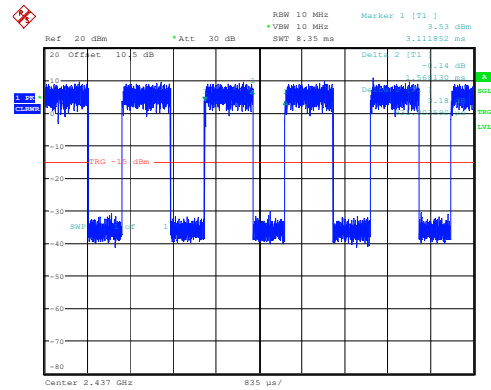
802.11n40_2437MHz
