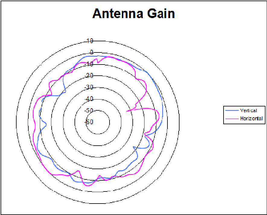
Antenna Pattern (5825MHz):
