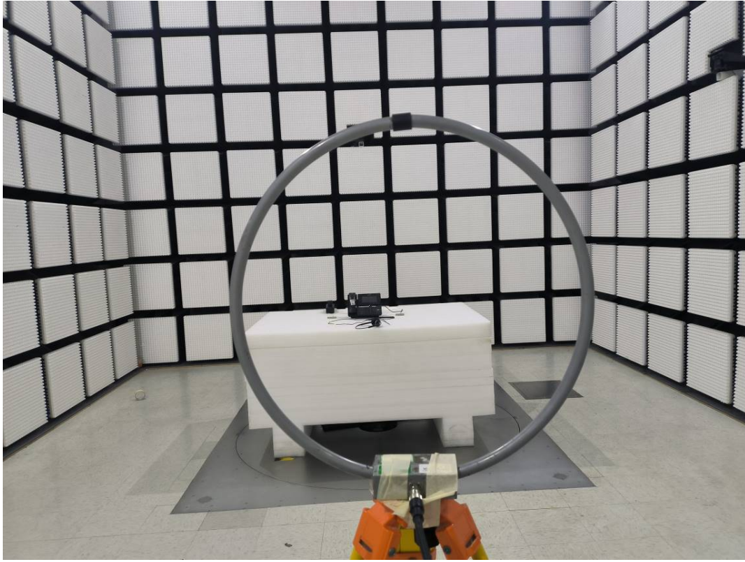
Radiated Emission 9k-30MHz View Perpendicular For Adapter 1
