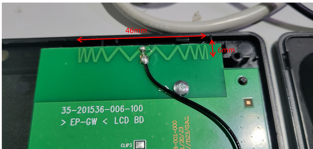
Antenna 1 Dimensions:
