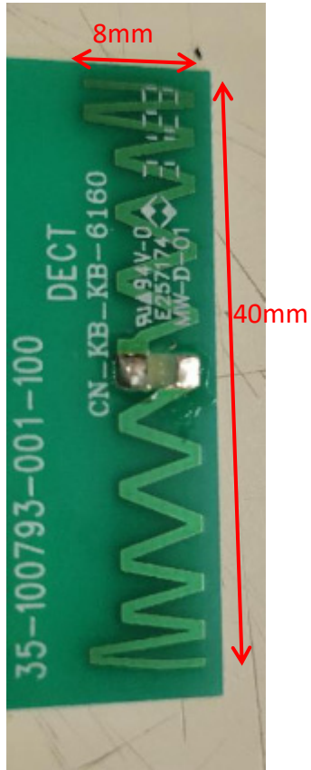
Antenna 1 Dimensions:
