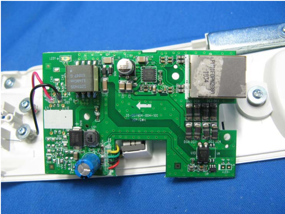
PoE Cradle Main PCB comp side
