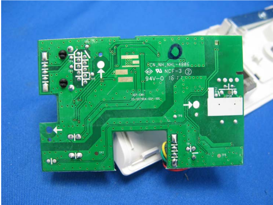
PoE Cradle Main PCB solder side
