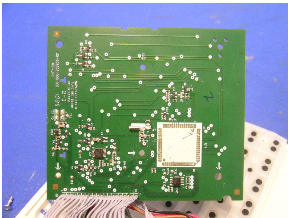
Base Unit Keypad rear side (View 2)
