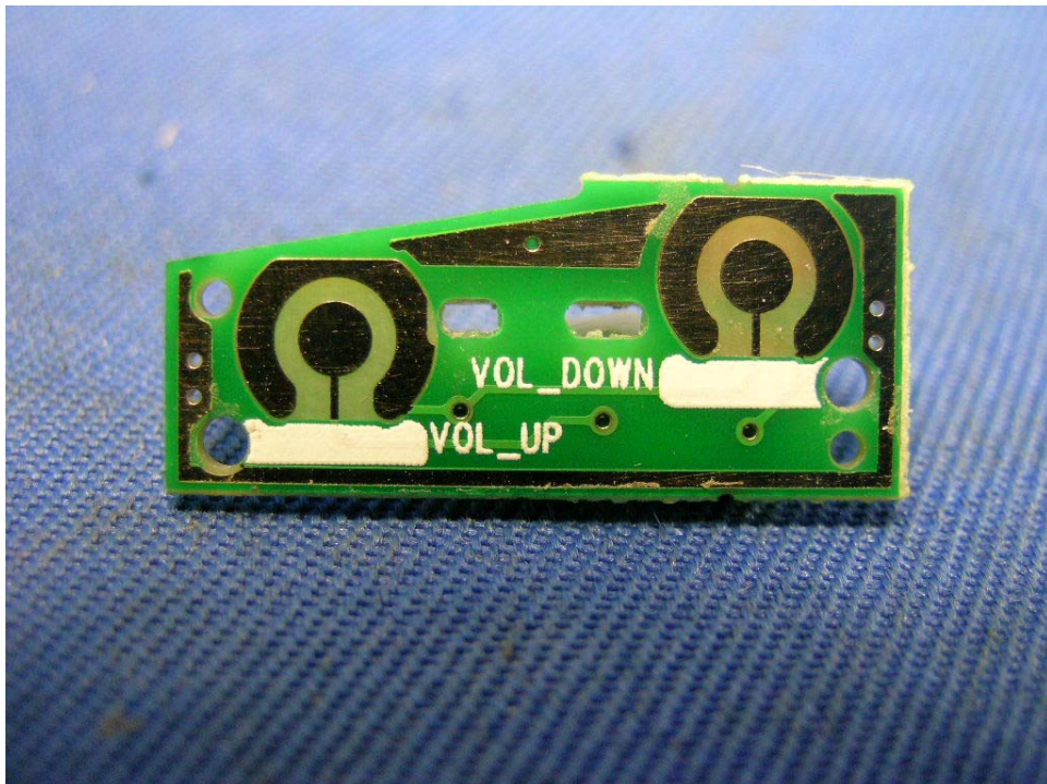
Handset Volume Key front side
