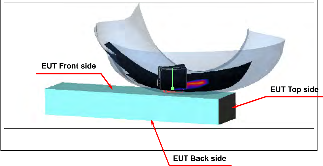
Figure 4. Left Head SAR Test Setup (Cheek)
