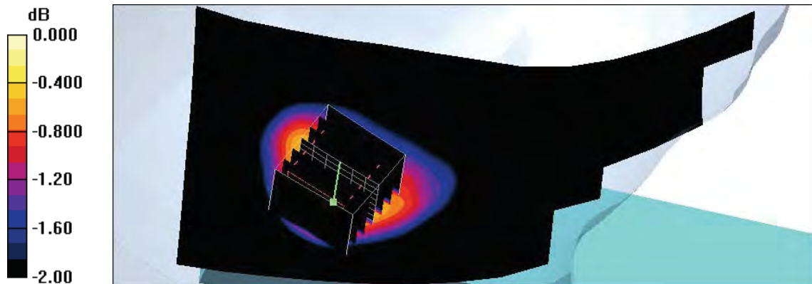
0 dB = 0.022mW/g
