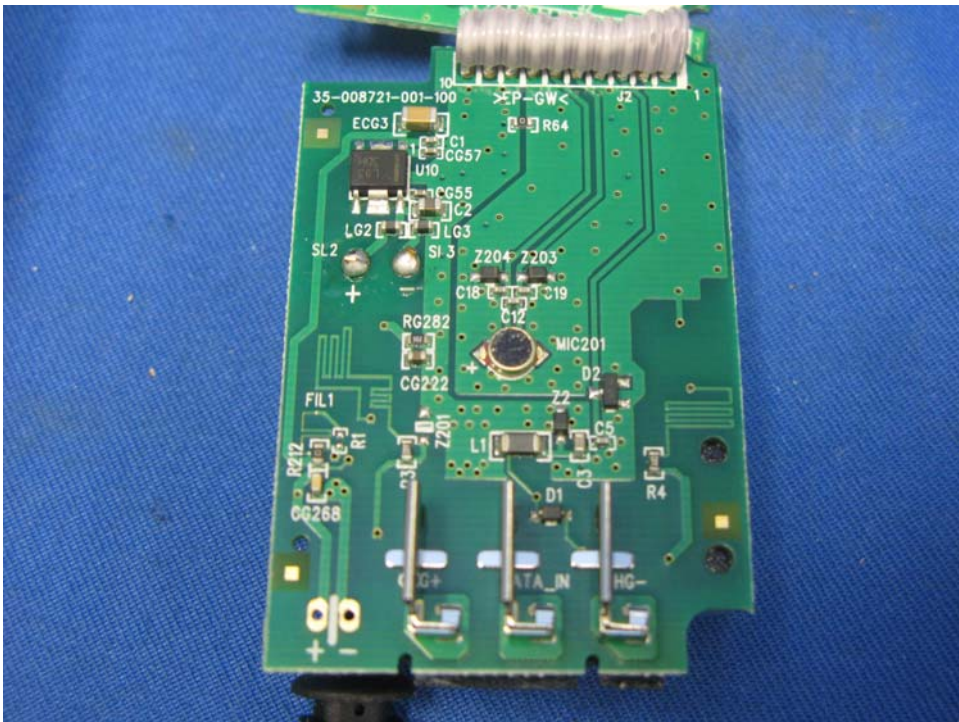
Handset Charging Board front side
