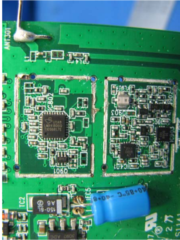
Base Unit Oscillator PCB comp side (View 1)
