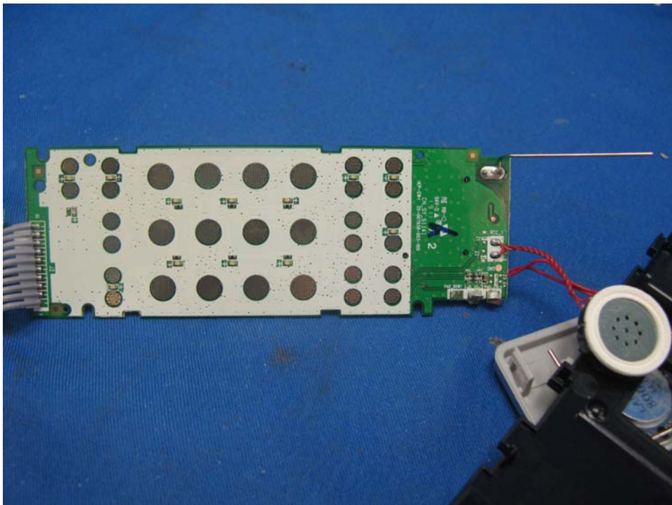
Handset Unit Main PCB solder side
