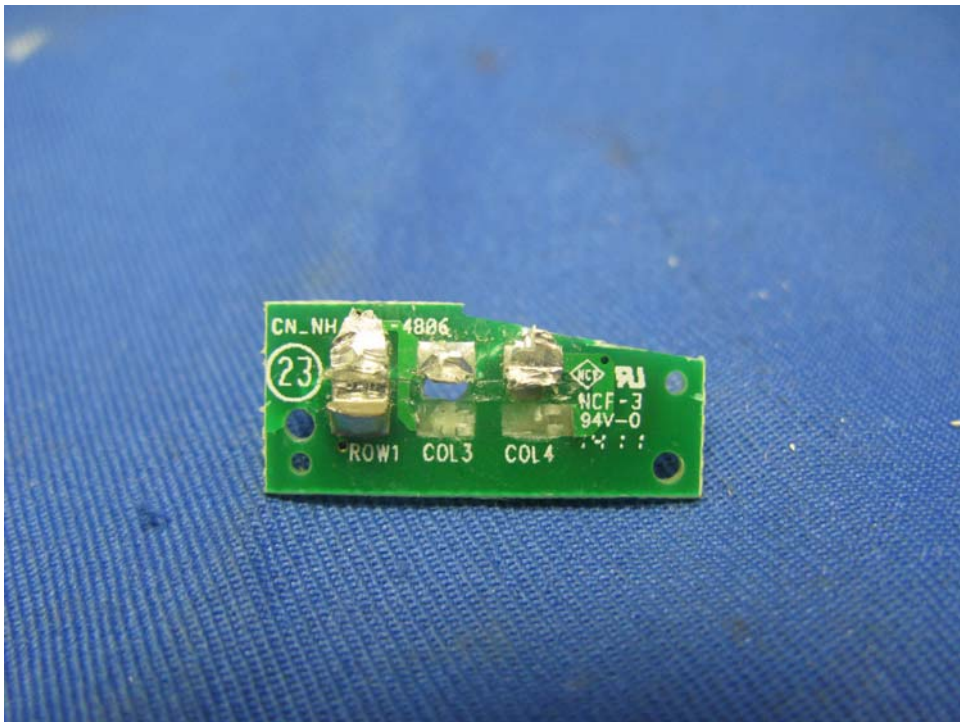
Handset Unit Volume Key rear side
