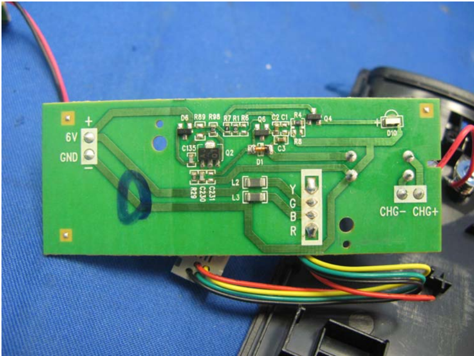
Cradle Main PCB comp side
