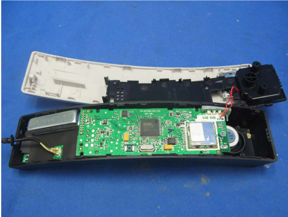
Handset Unit assembly
