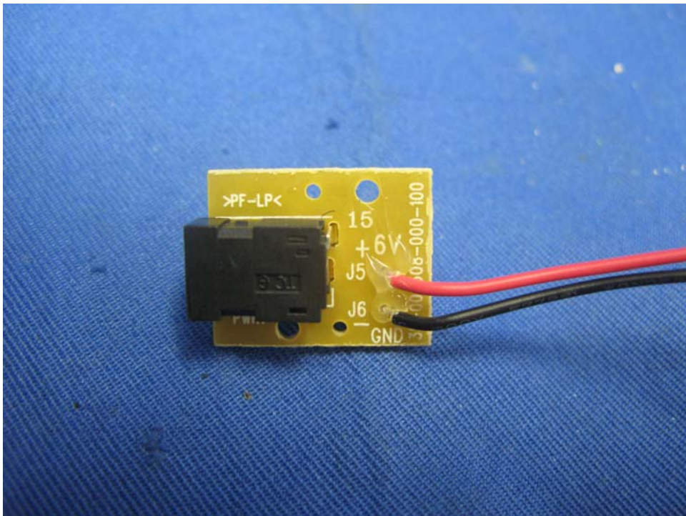
Cradle AC Jack front side
