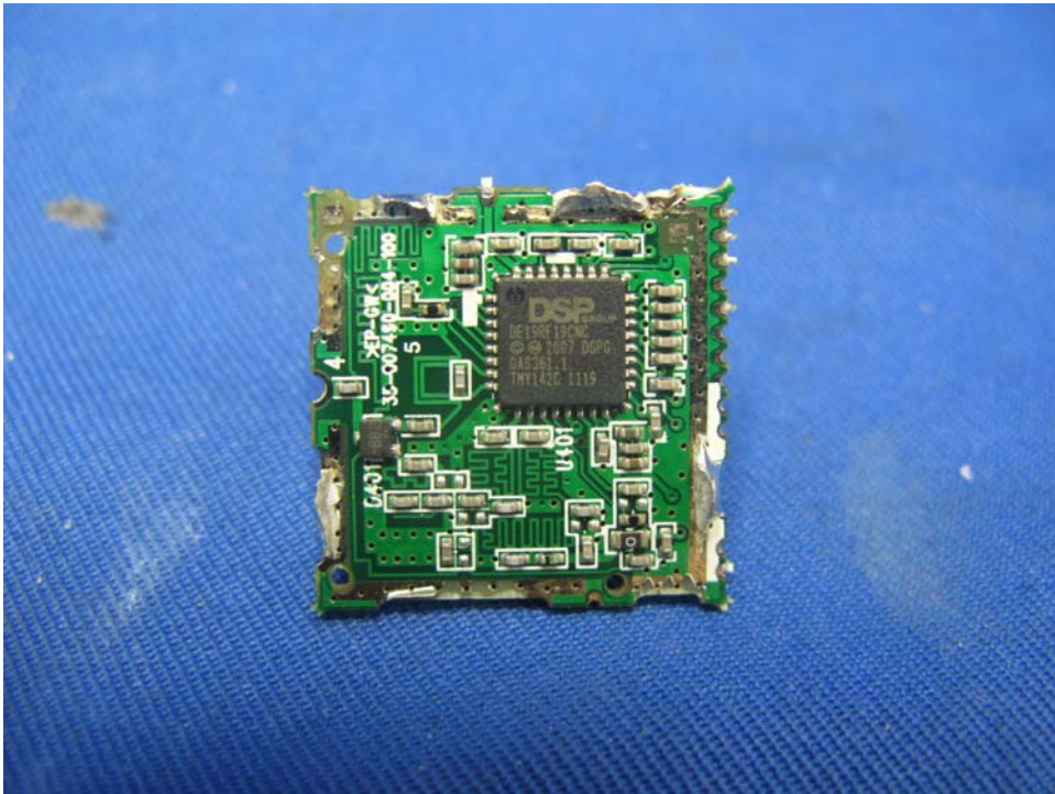
Handset Unit Oscillator PCB comp side
