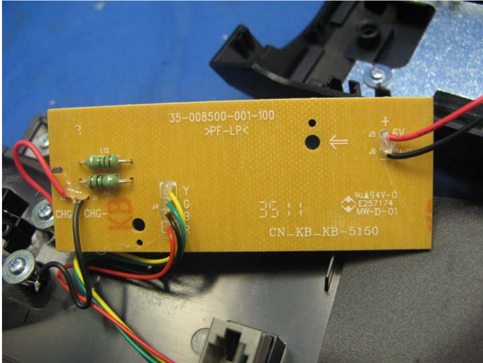
Cradle Main PCB solder side
