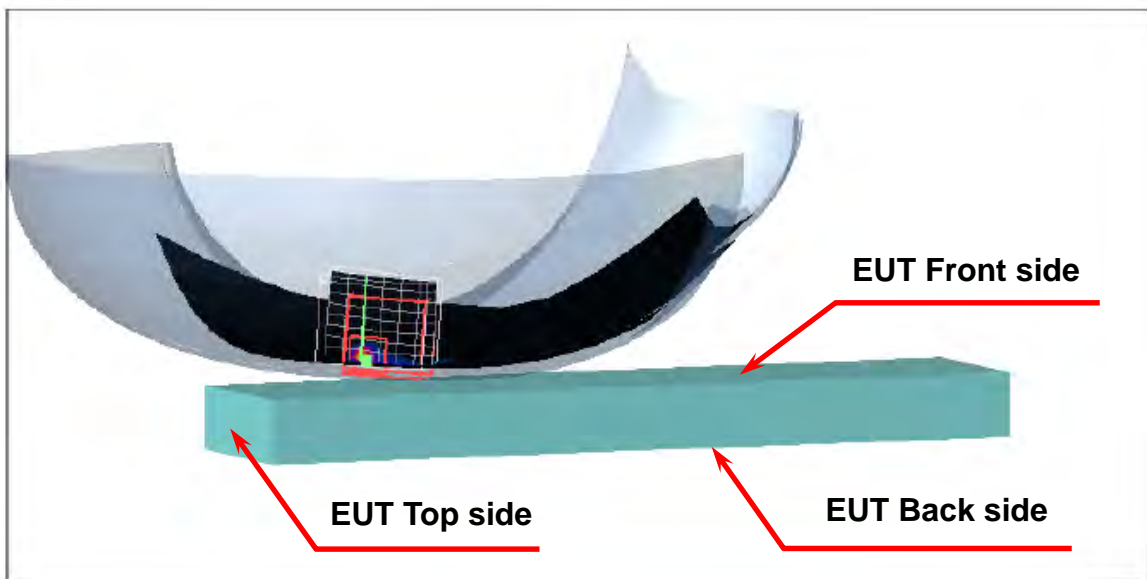
Figure 2. Right Head SAR Test Setup (Cheek)
