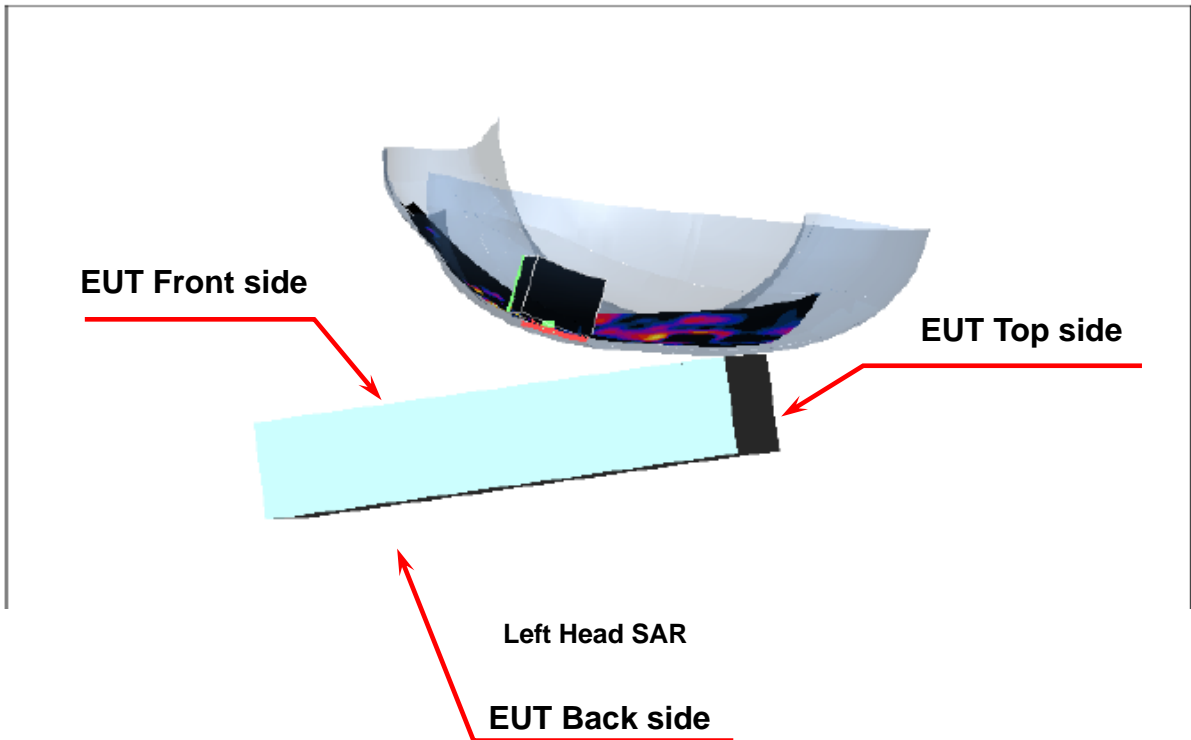
Figure 4. Left Head SAR Test Setup (Cheek)
