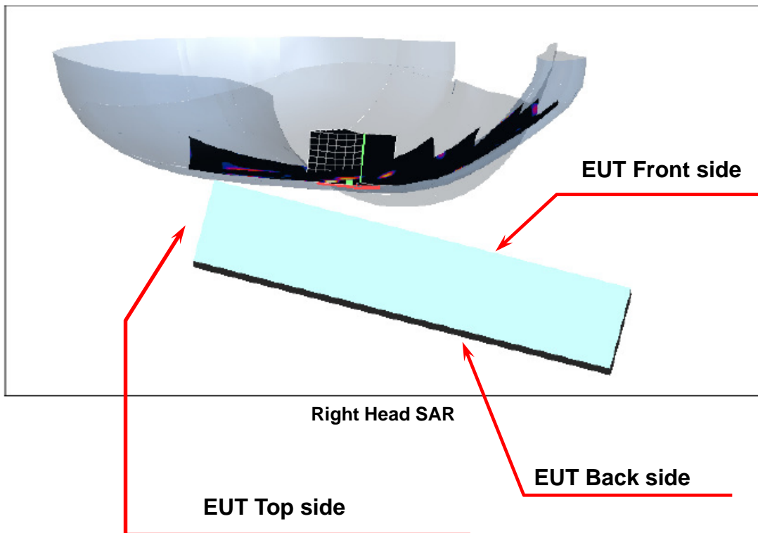
Figure 2. Right Head SAR Test Setup (Cheek)
