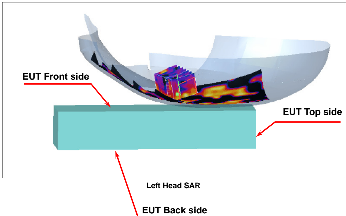
Figure 4. Left Head SAR Test Setup (Cheek)
