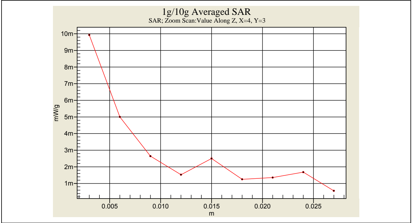
Head SAR Measurement _ Right-Tilted CH2 (LINE 1)
