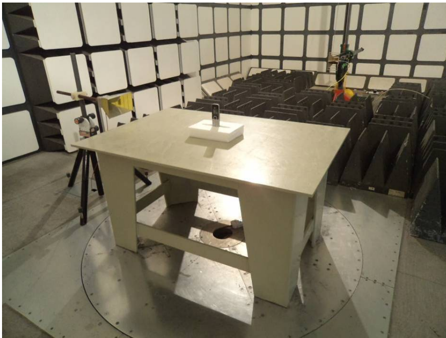
Radiated Emissions View (Above 1 GHz, 2# Handset)
