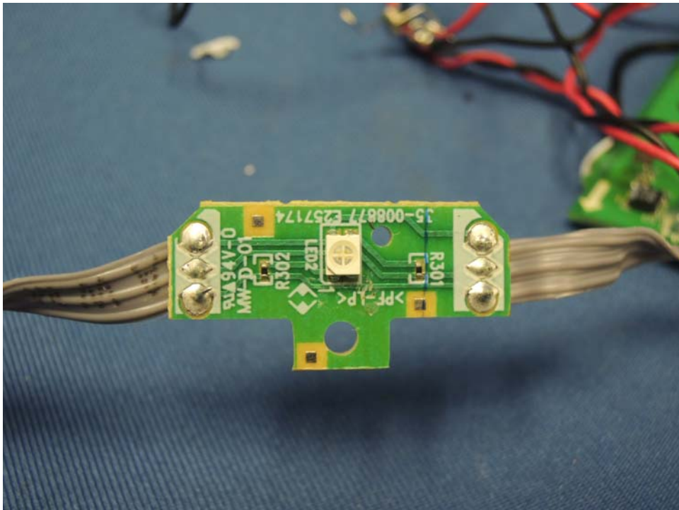
Base Unit LED 4 front side
