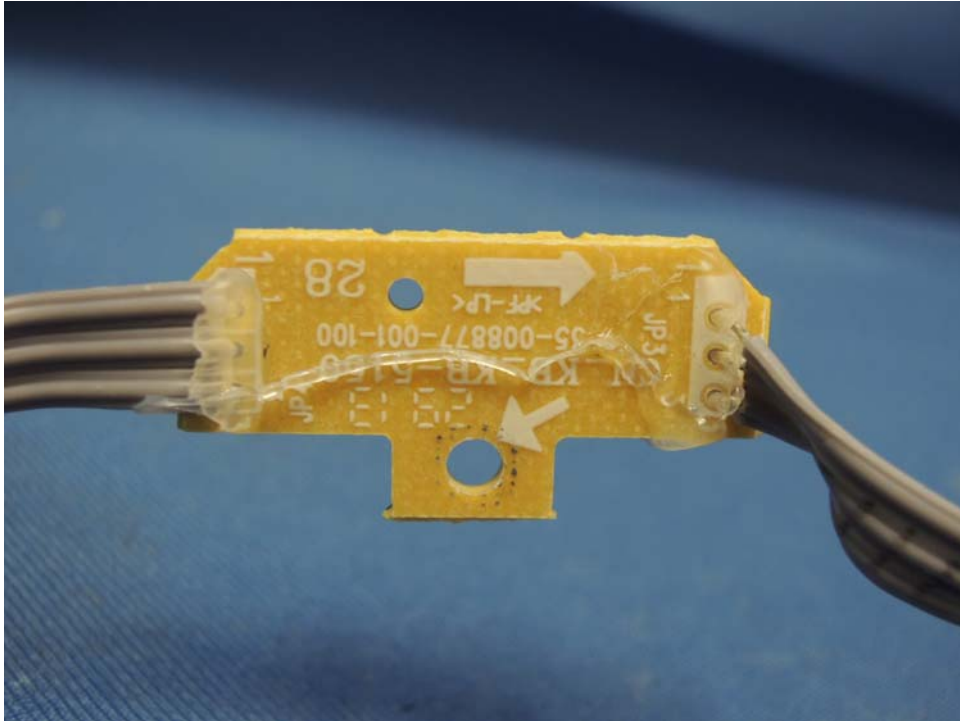
Base Unit LED 2 rear side
