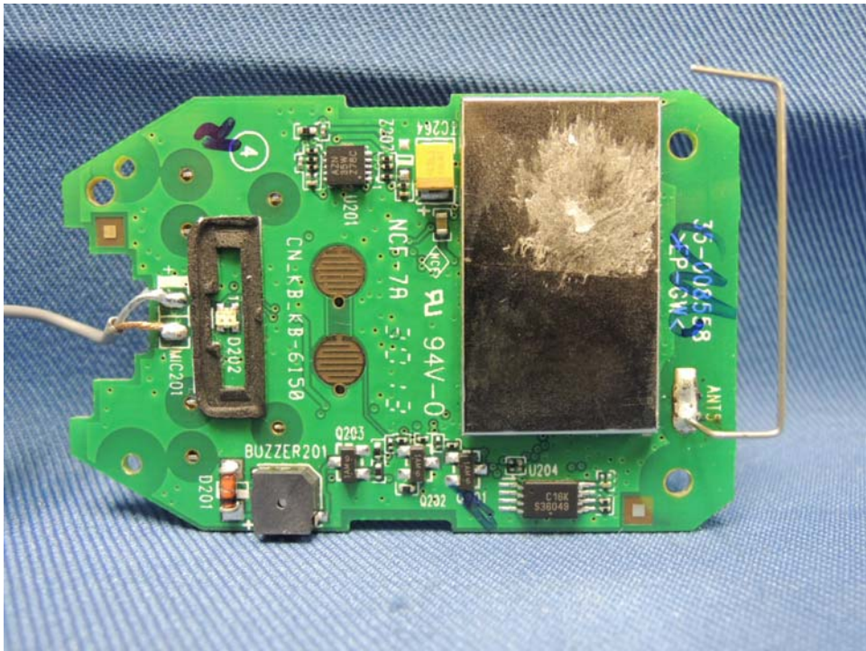
Mic. Unit Main PCB comp side
