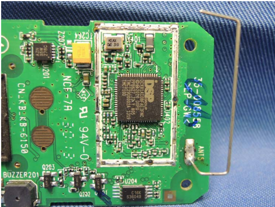
Mic. Unit Oscillator PCB comp side
