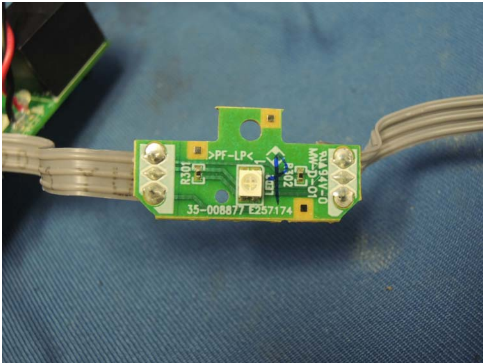
Base Unit LED 2 front side
