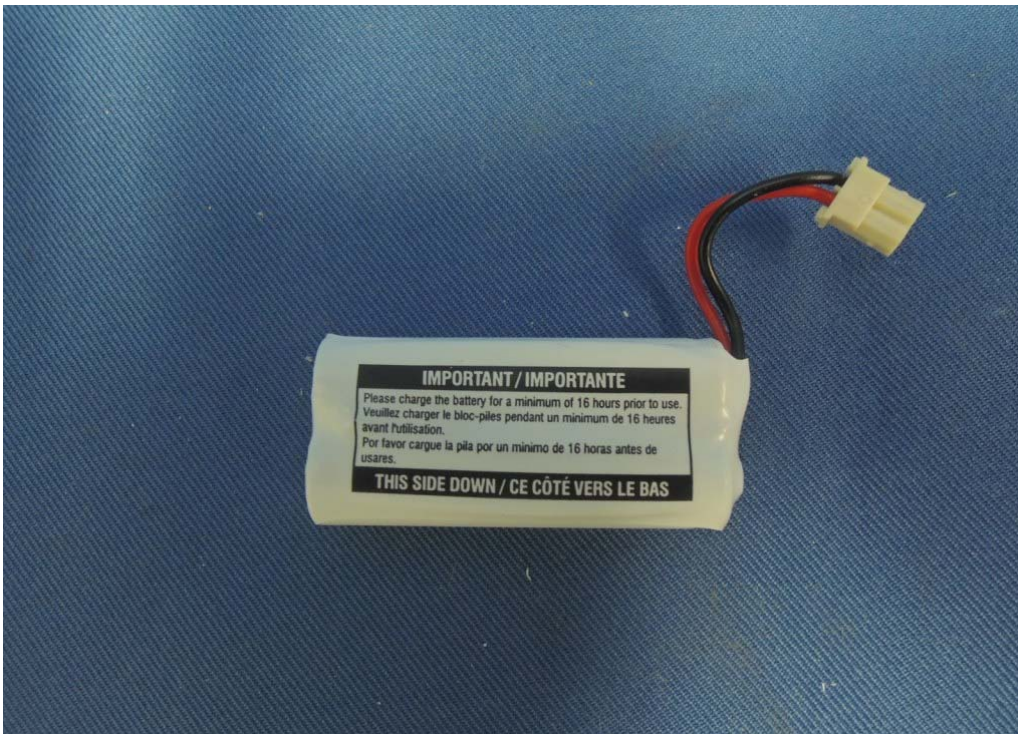
Figure 8 – 2.4VDC 300mAh Coslight battery back view
