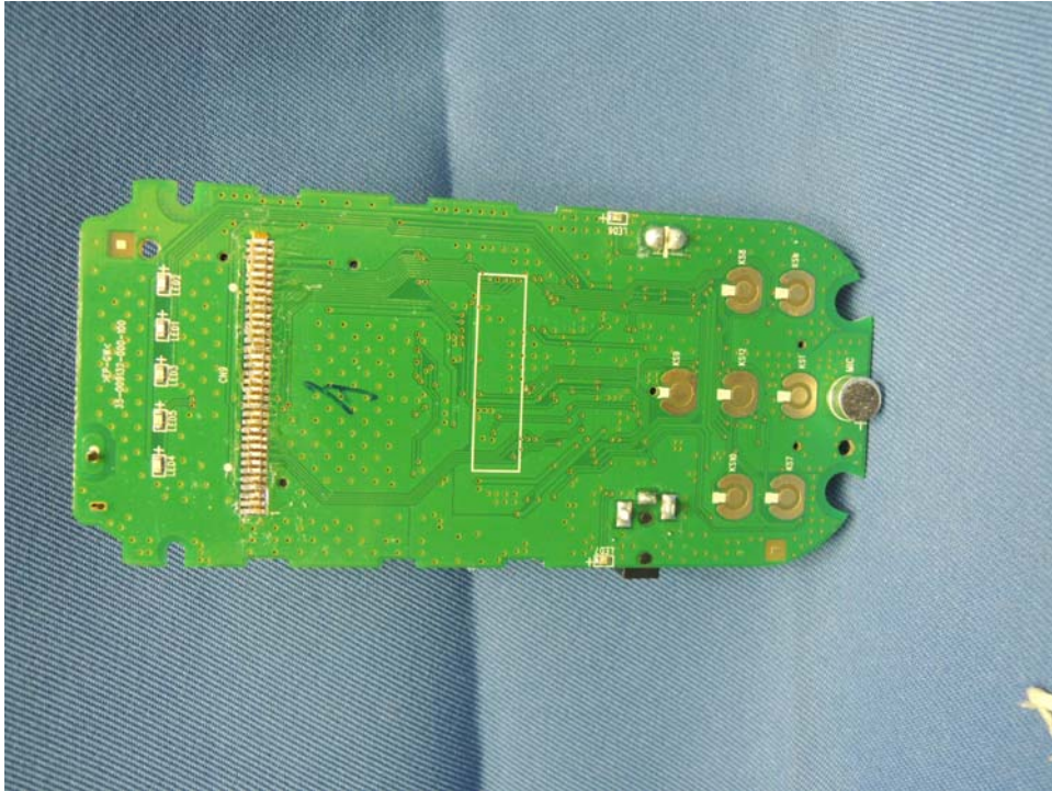
Parent Unit Main PCB solder side (View 2)
