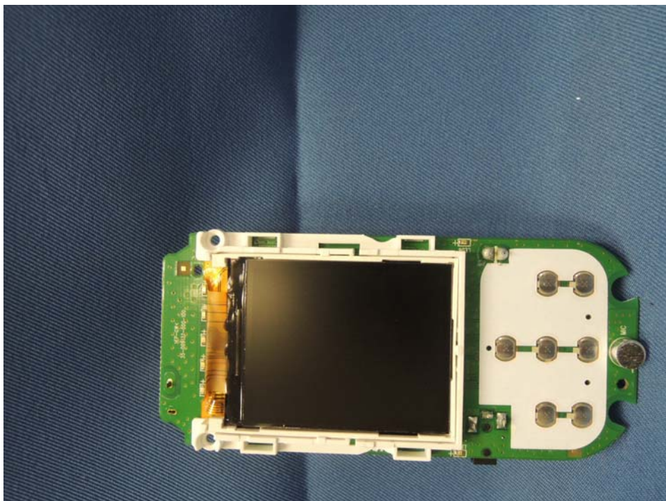
Parent Unit Main PCB solder side (View 1)
