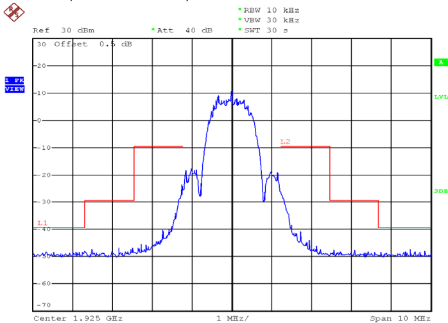
Deskset unit, Middle channel, Traffic carrier
