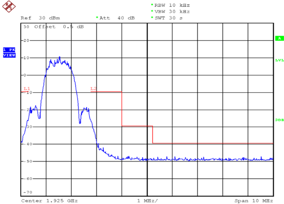
Deskset unit, Lowest channel, Traffic carrier
