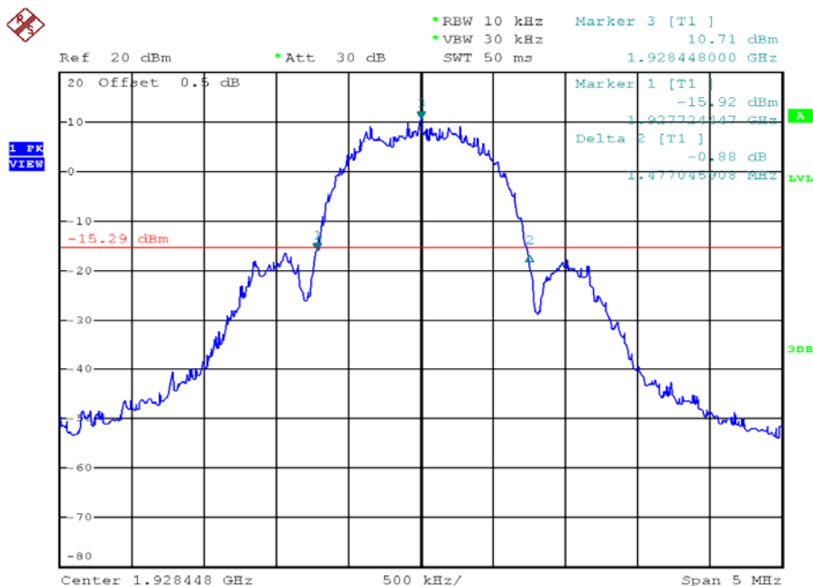
Deskset unit, Highest channel, Traffic carrier
