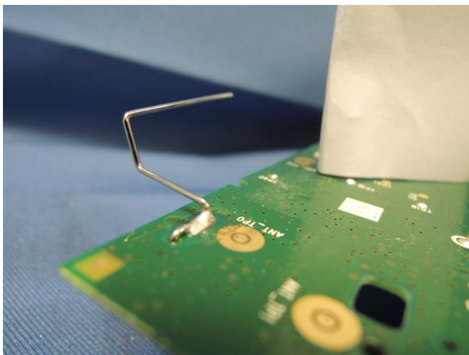
Base Unit DECT Antenna 0
