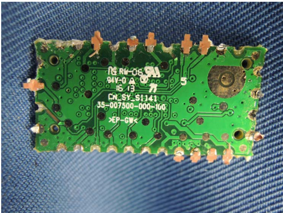
Base Unit Bluetooth Module solder side
