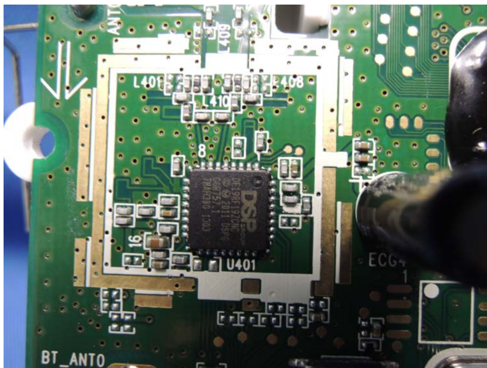
Base Unit DECT RF Module PCB comp side
