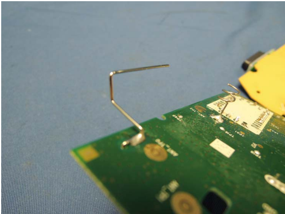
Base Unit DECT Antenna 0 and Bluetooth Antenna
