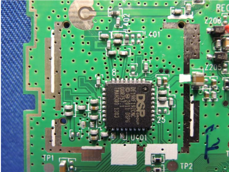
Handset DECT RF Module PCB comp side
