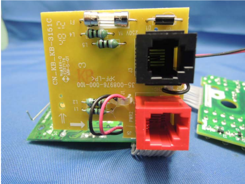
Base Unit Telephone Line and AC Line Jack front side
