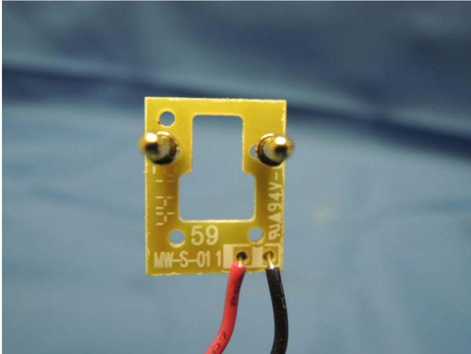
Base Unit Charging Pad front side
