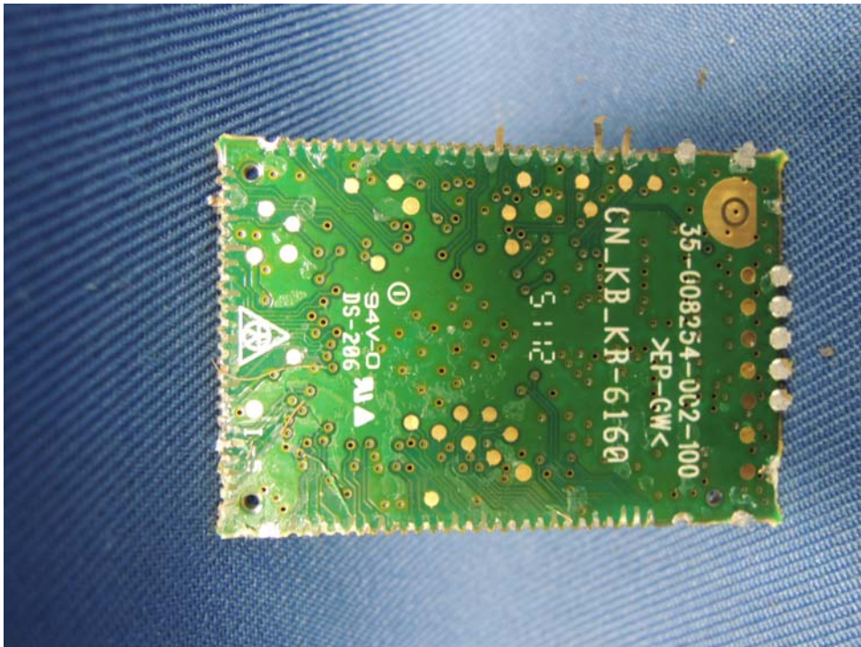
Base Unit DECT Module rear side
