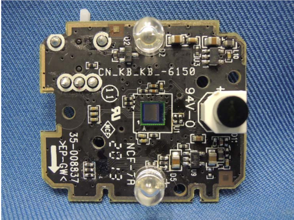
Baby Unit Camera PCB front side (View 2)
