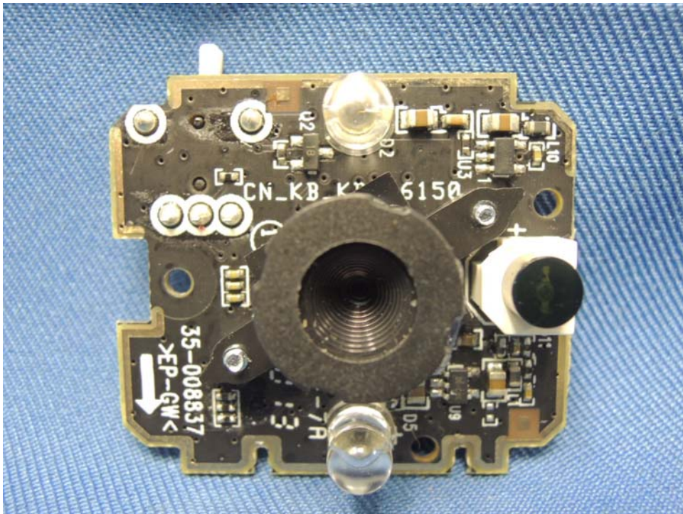
Baby Unit Camera PCB front side (View 1)
