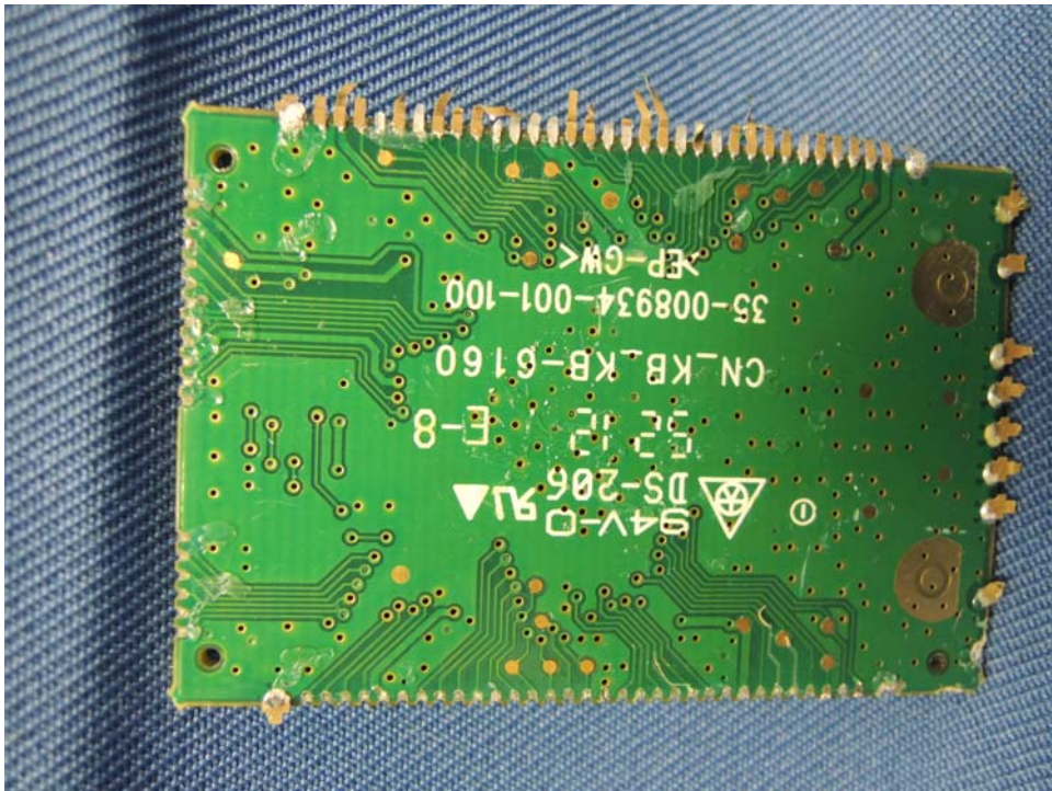
Base Unit DECT Module PCB rear side
