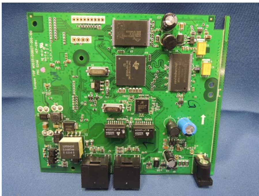
Deskset Main PCB comp side (View 2)
