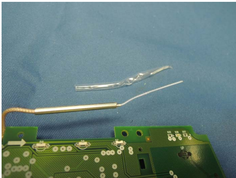
Deskset Antenna (View 2)
