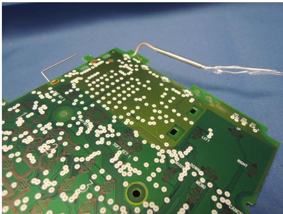
Deskset Antenna (View 1)
