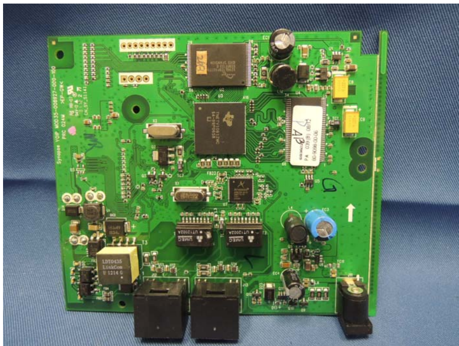
Deskset Main PCB comp side (View 1)
