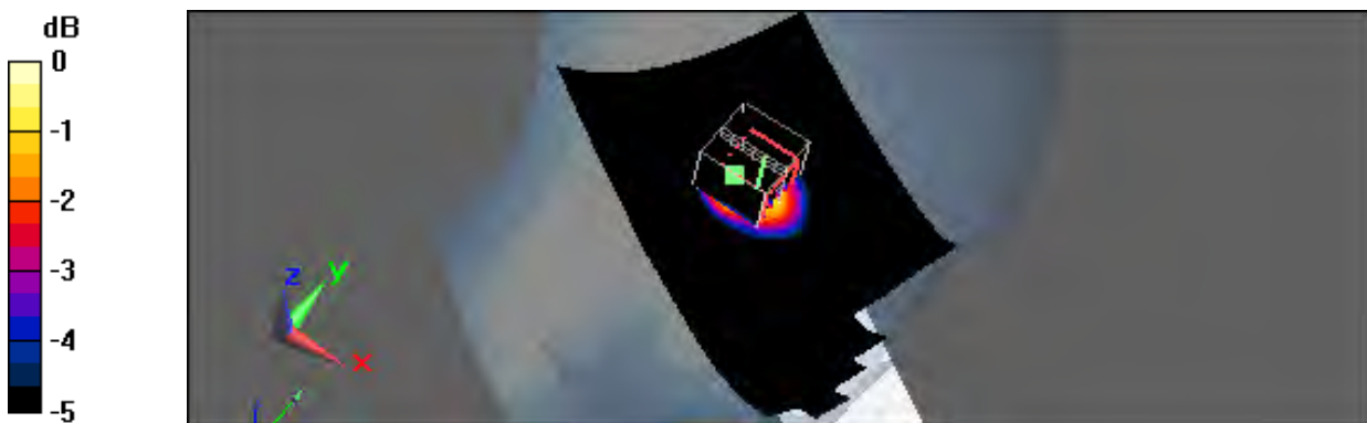
0 dB = 0.057mW/g
