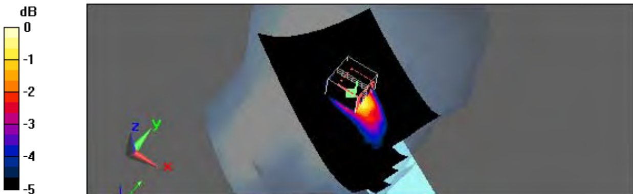
0 dB = 0.070mW/g
