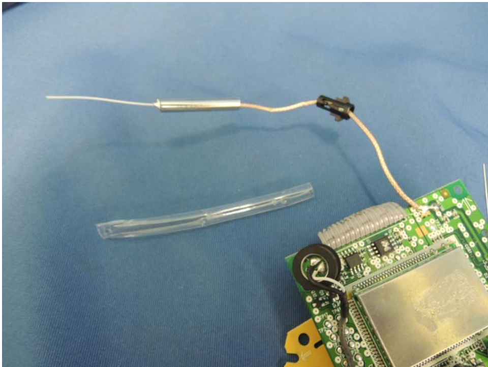
Base Unit 2 nd Antenna
