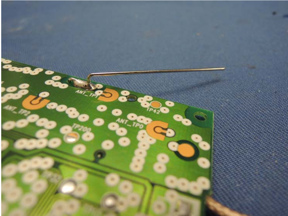
Base Unit 1 st Antenna
