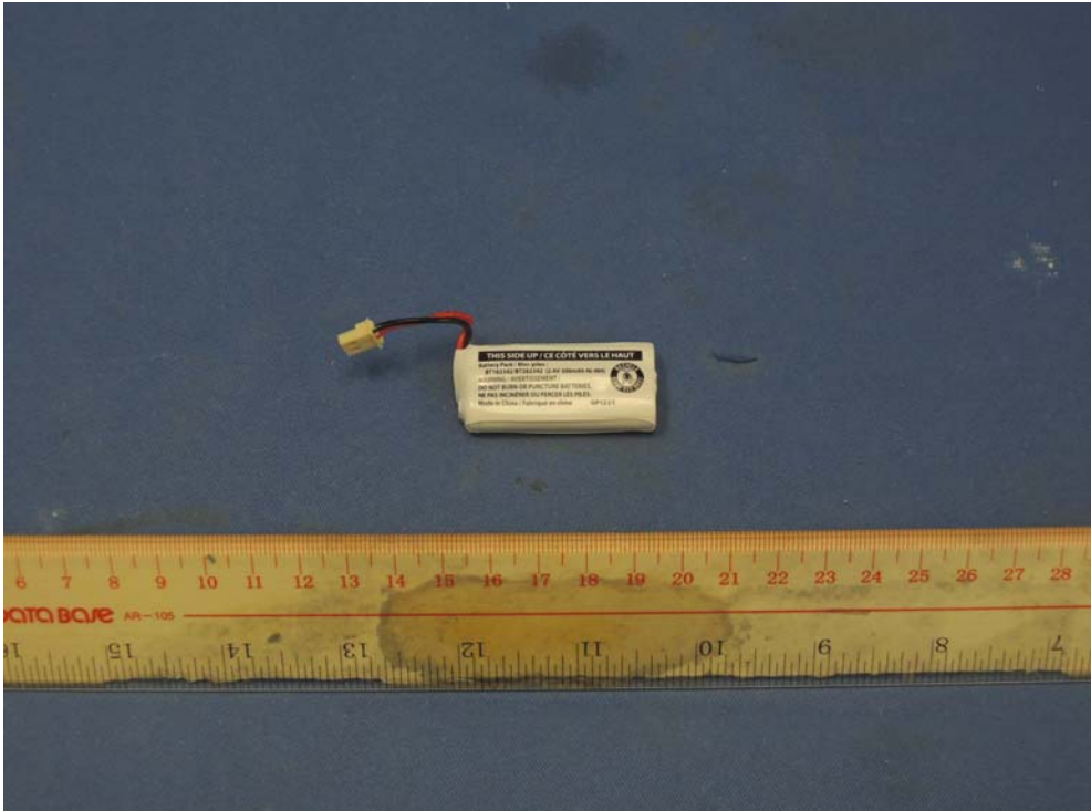
Figure 5 – 2.4VDC 300mAh GPI rechargeable battery front view
