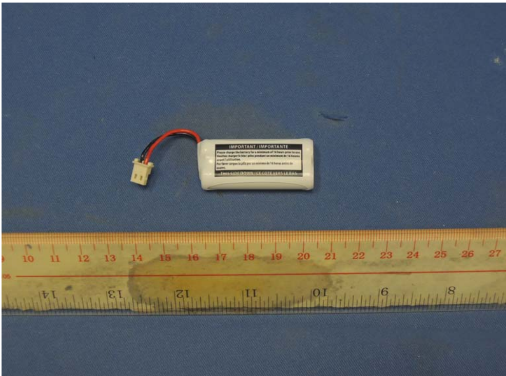
Figure 4 – 2.4VDC 300mAh CORUN rechargeable battery back view
