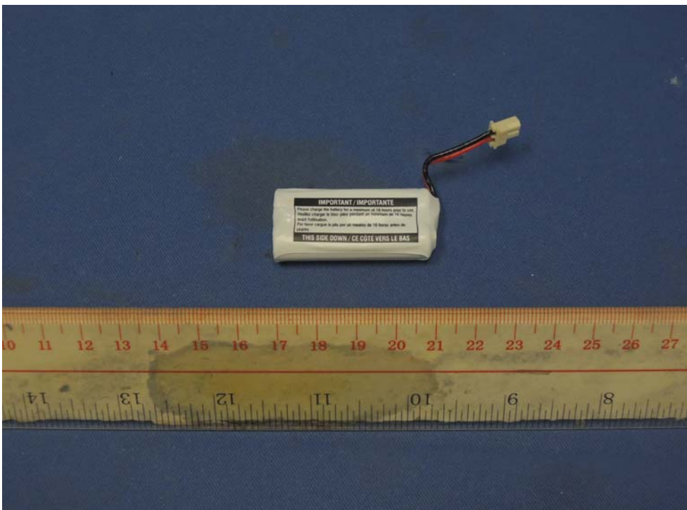
Figure 10 – 2.4VDC 300mAh Coslight rechargeable battery back view
