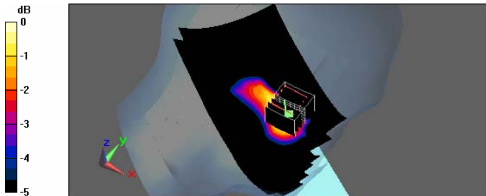
0 dB = 0.037mW/g
