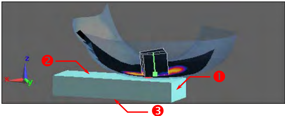
Figure 4. Left Head SAR Test Setup (Cheek)
