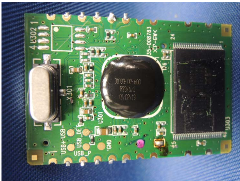
Base Unit RF Module front side
