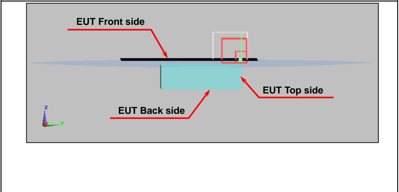
Figure 2. Brain SAR Test Setup (Flat Section)
