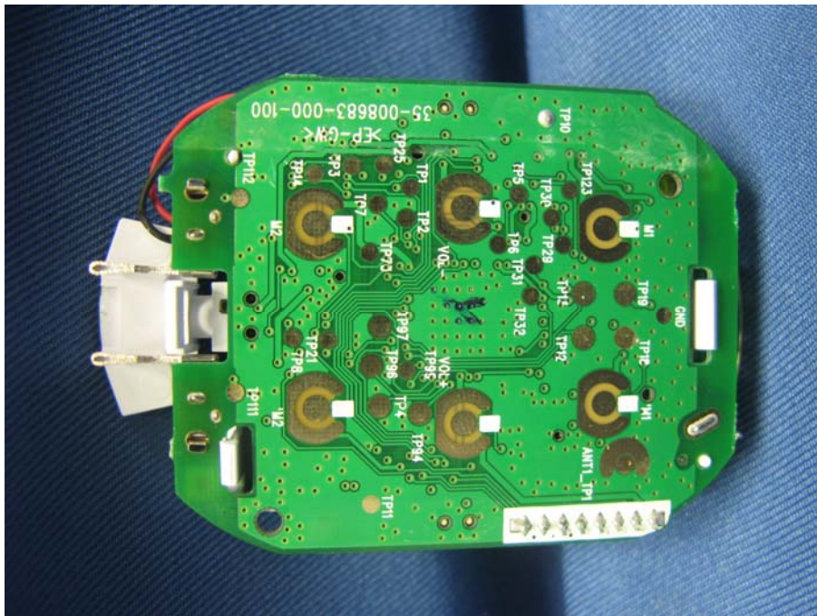
Pendant Main PCB solder side
