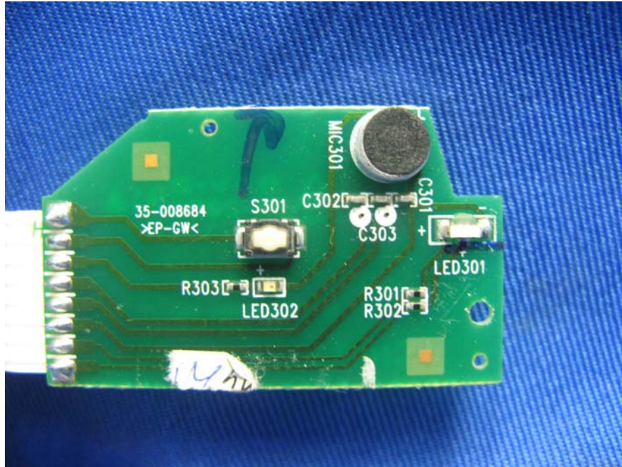
Pendant LED & Mic. front side
