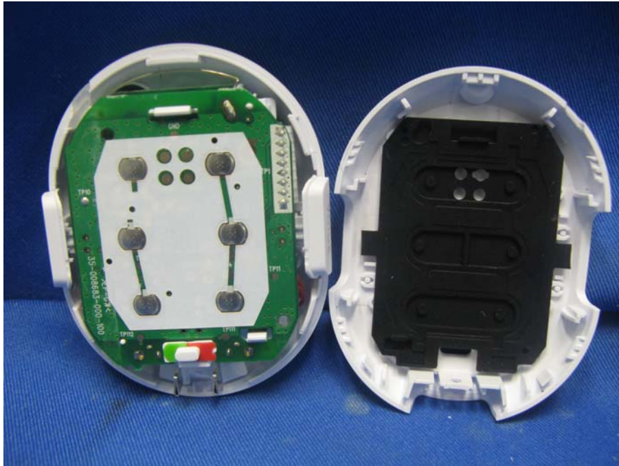
Pendant assembly (View 1)
