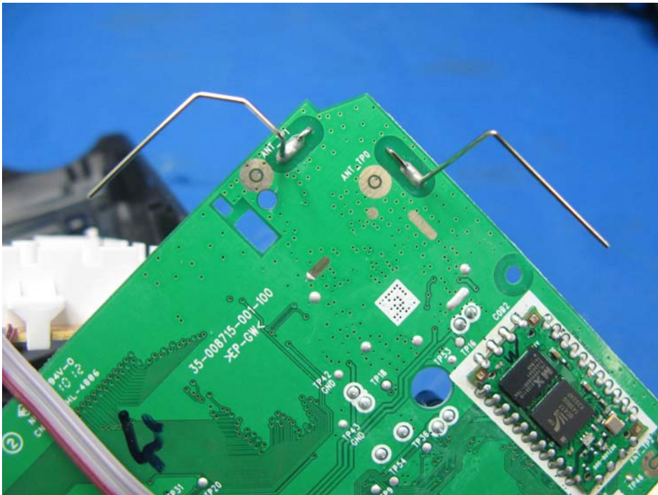
Base Unit DECT Antenna
