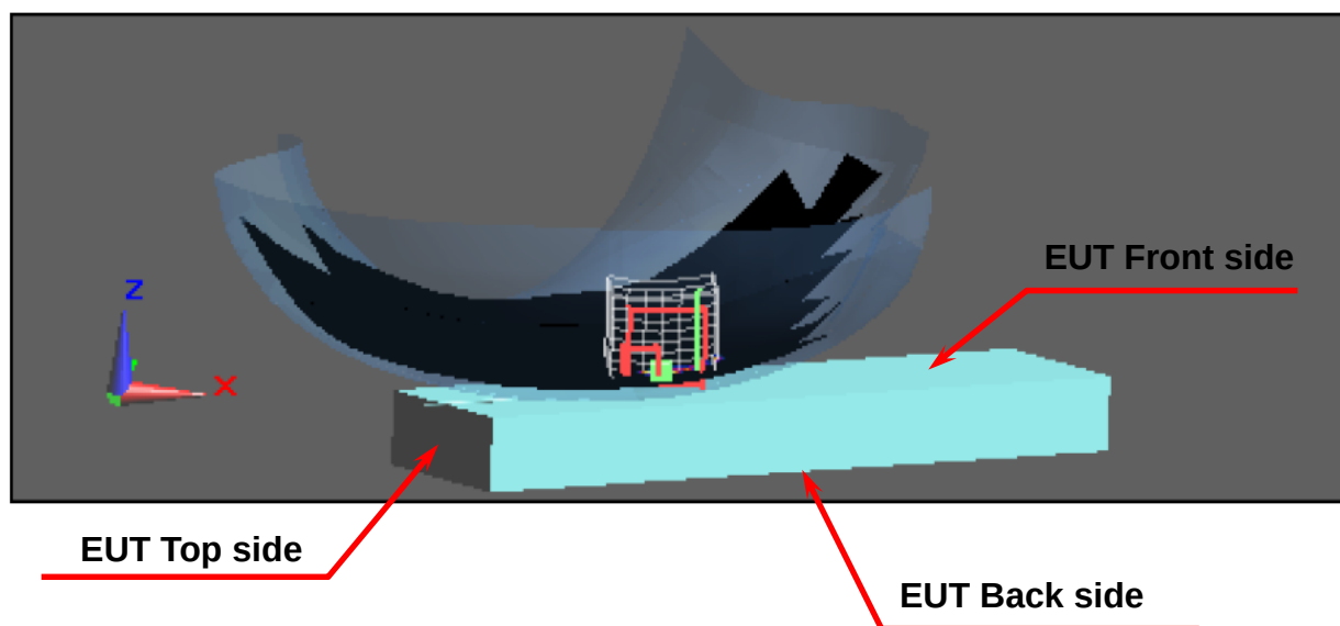
Figure 2. Right Head SAR Test Setup (Cheek)
