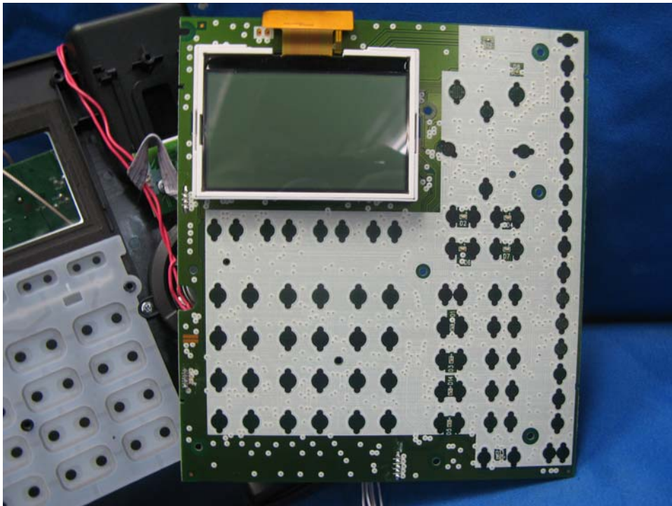
Base Unit LCD Display and Keypad front side (View 1)
