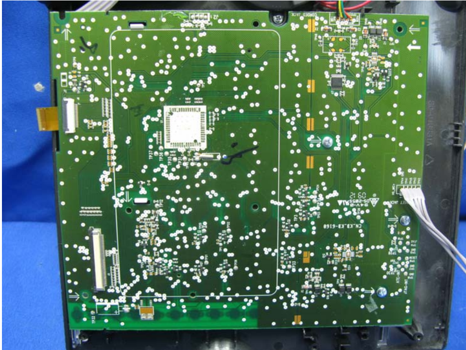
Base Unit LCD Display and Keypad rear side (View 2)
