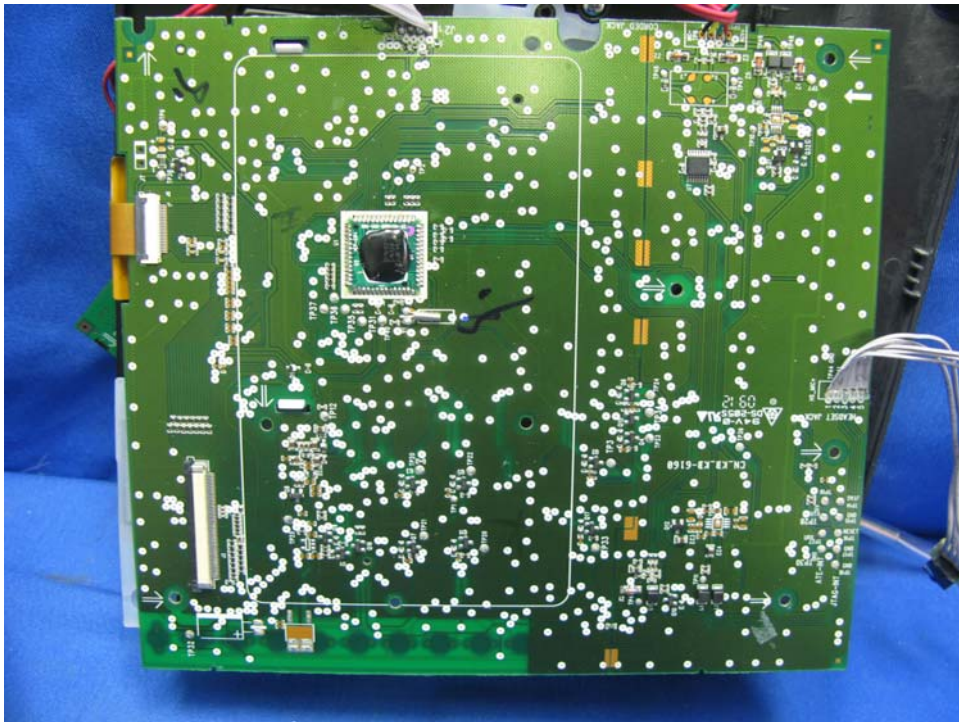
Base Unit LCD Display and Keypad rear side (View 1)
