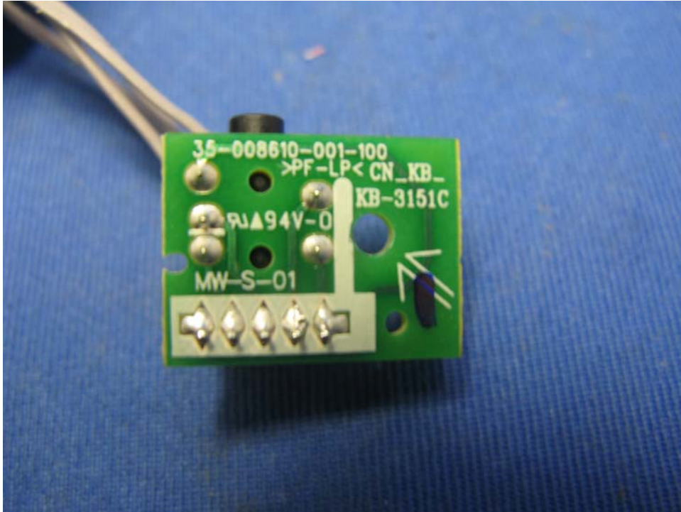
Base Unit Headset Jack rear side
