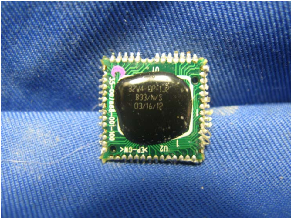
Base Unit Keyboard Controller IC front side
